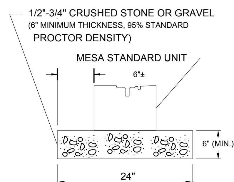
1 TYPICAL TIERED CROSS-SECTION
