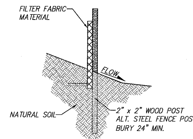
SILT FENCE FOR SEDIMENT CONTROL SCALE: 1"=2'
