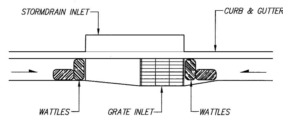
WATTLE DETAIL AT STORM INLET SCALE: 1"=2'
