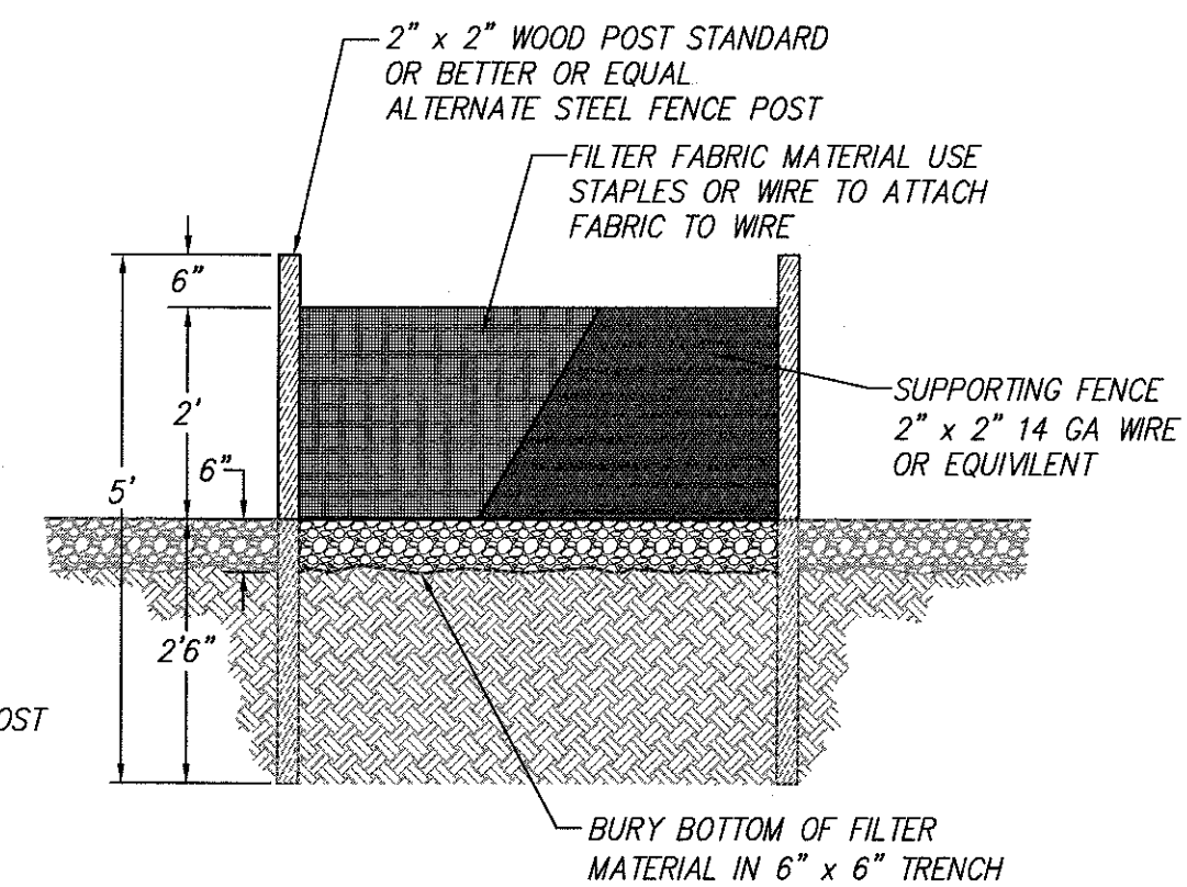
SILT FENCE FOR SEDIMENT CONTROL SCALE: 1"=2'
