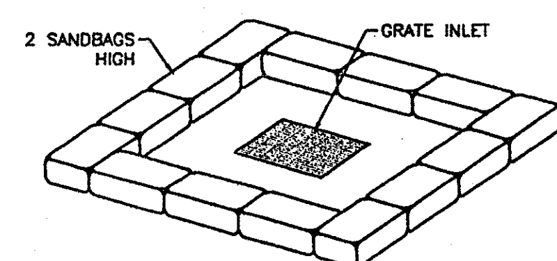
SANDBAG OR WATTLE DETAIL N.T.S.
