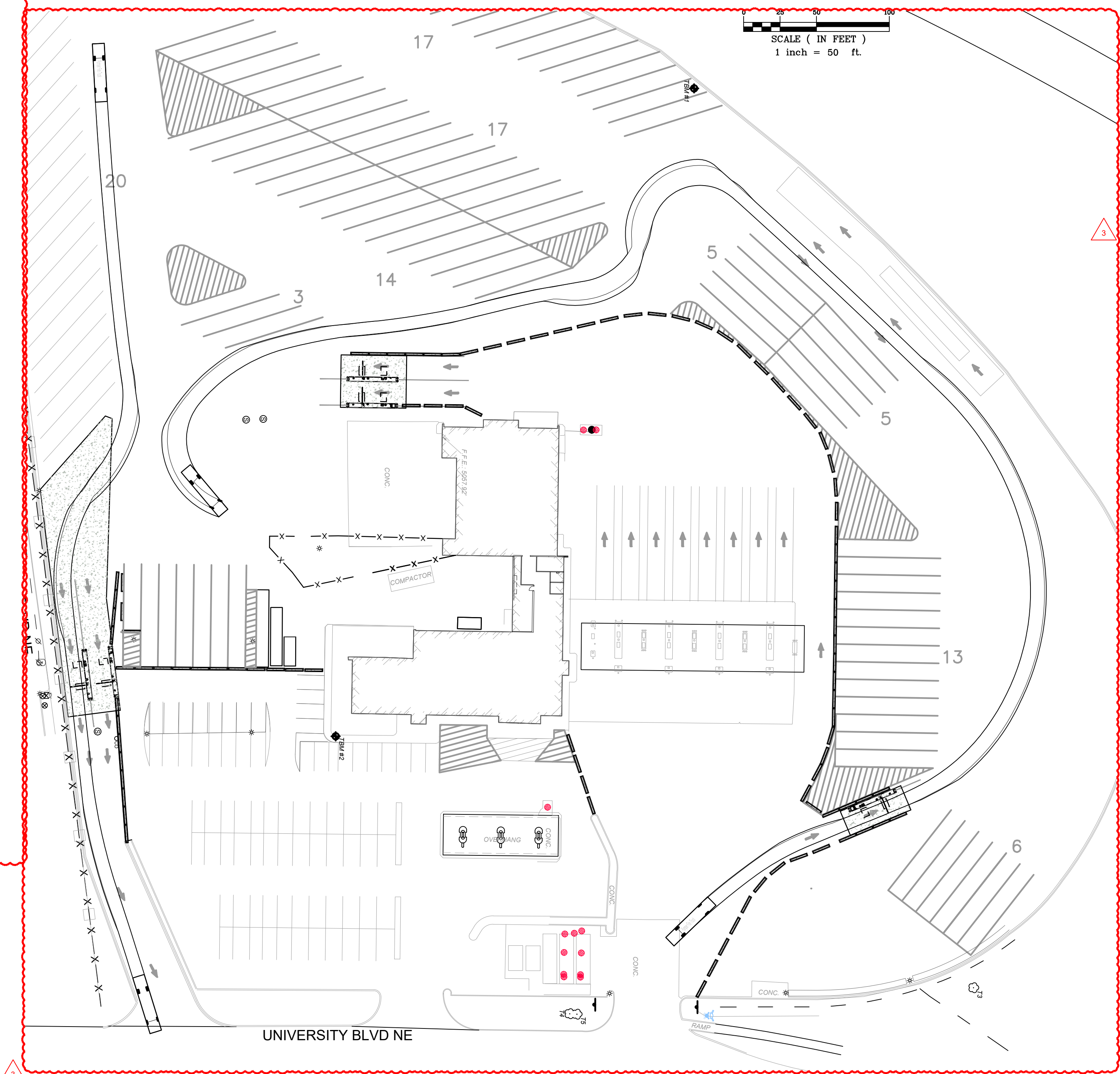
PUMPER FIRE TRUCK TURNING MOVEMENT 1 1" = 50' TT1.0
