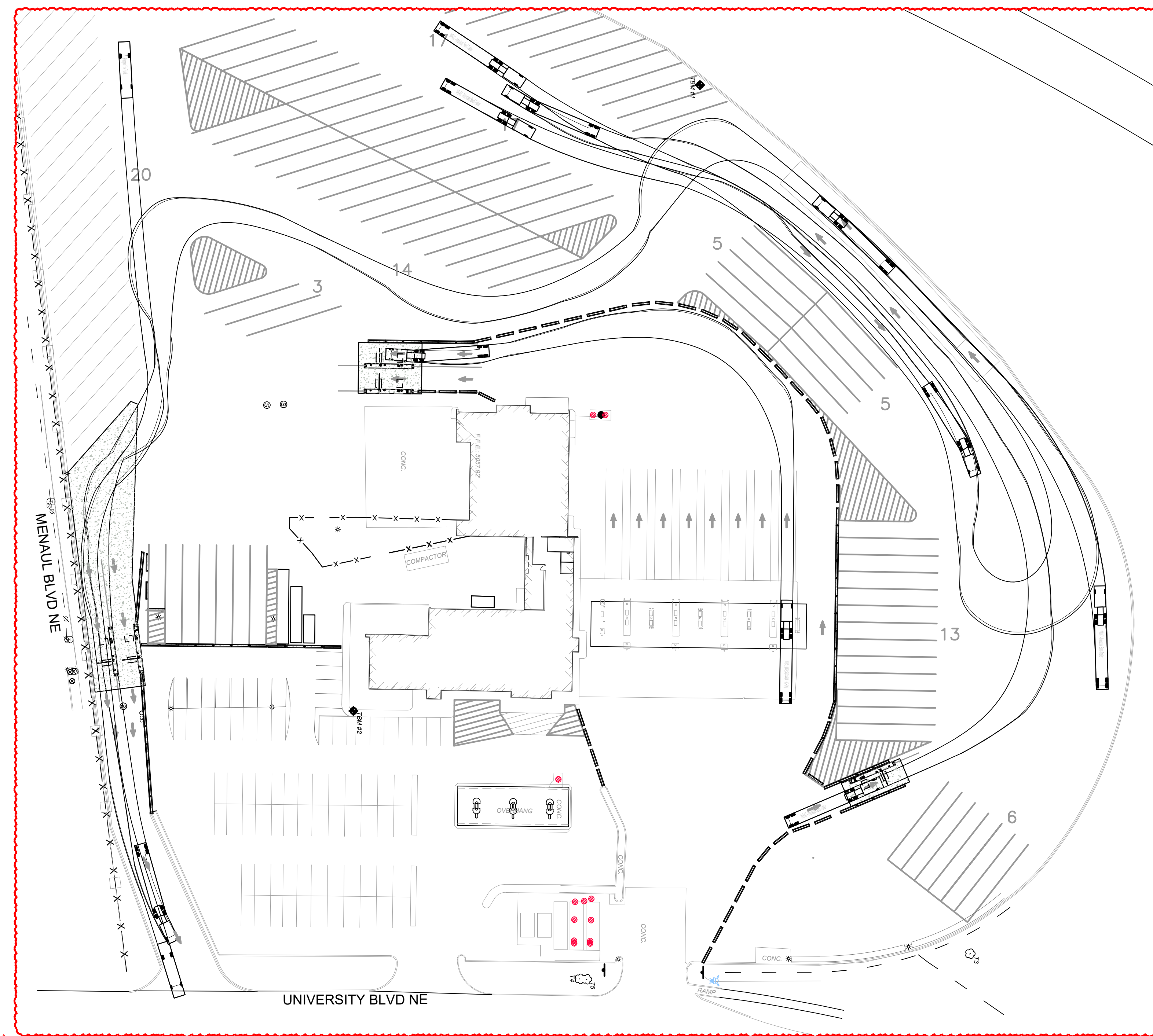
TRUCK TURNING MOVEMENT (WB-67 TRAILER) 1 TT10
