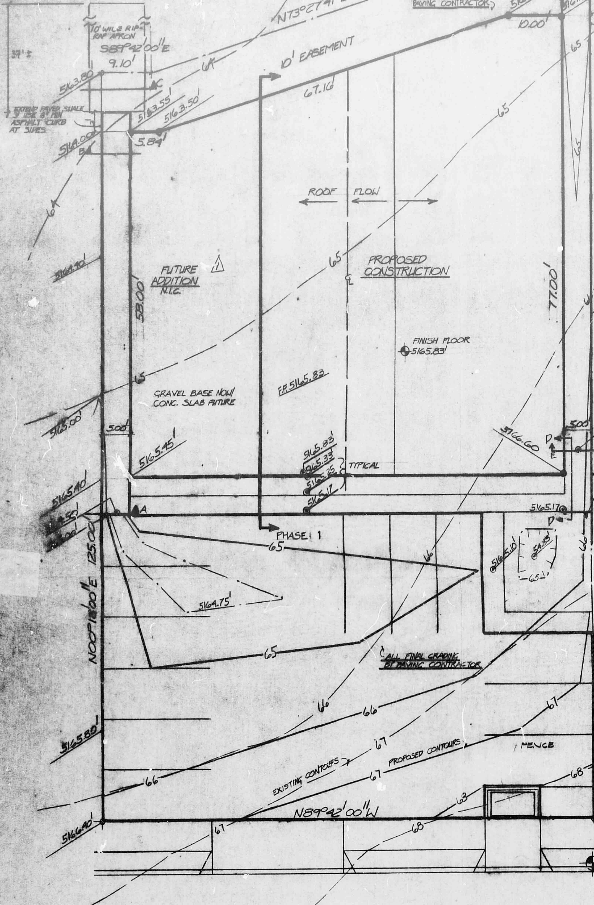
DRAINAGE PLAN 1"=10'-0"
