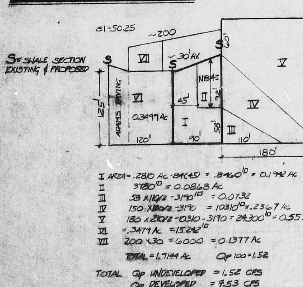
DRAINAGE PLAN 1"=10'-0"
