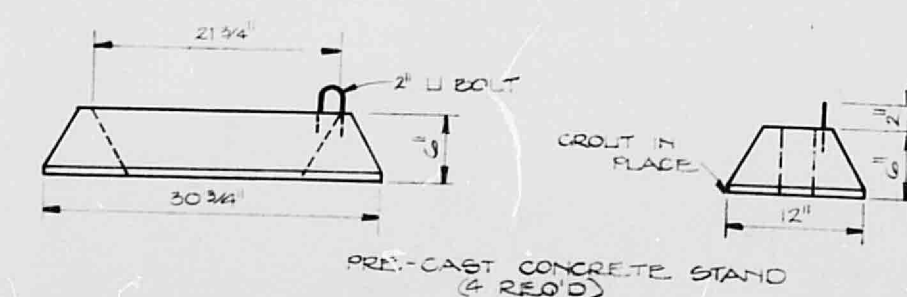
BICYCLE STAND SCALE: 3/4"=1'-0"
