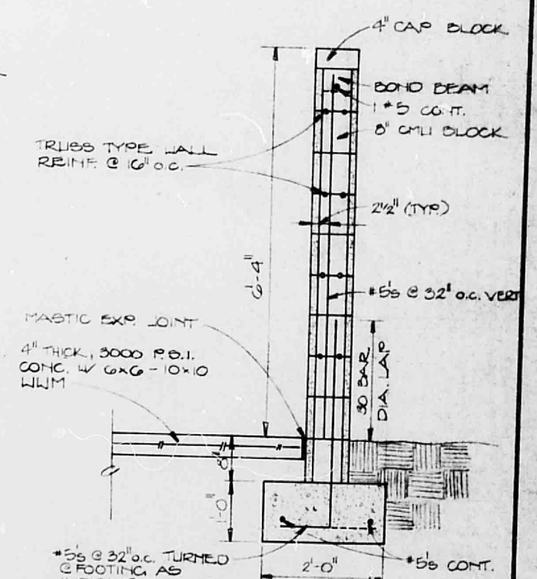
TRASH ENCLOSURE WALL SECT. SCALE: 1/2"=1'-0"
