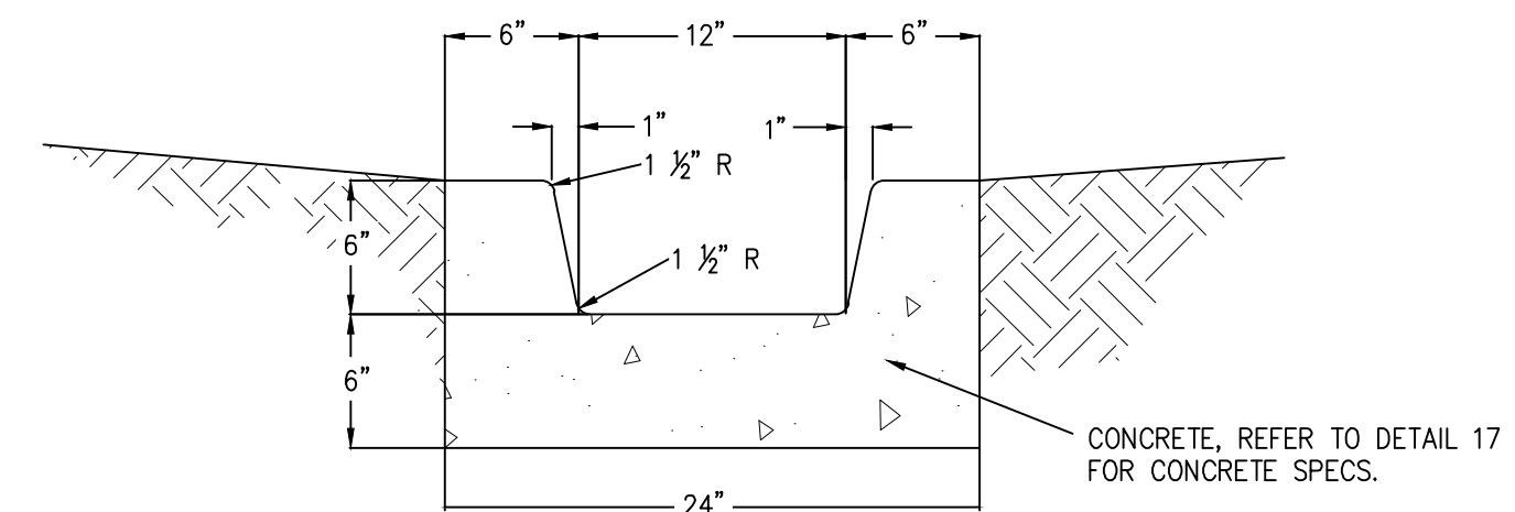
36 C-4.2 1' WIDE CURB CHASE DETAIL NOT TO SCALE
