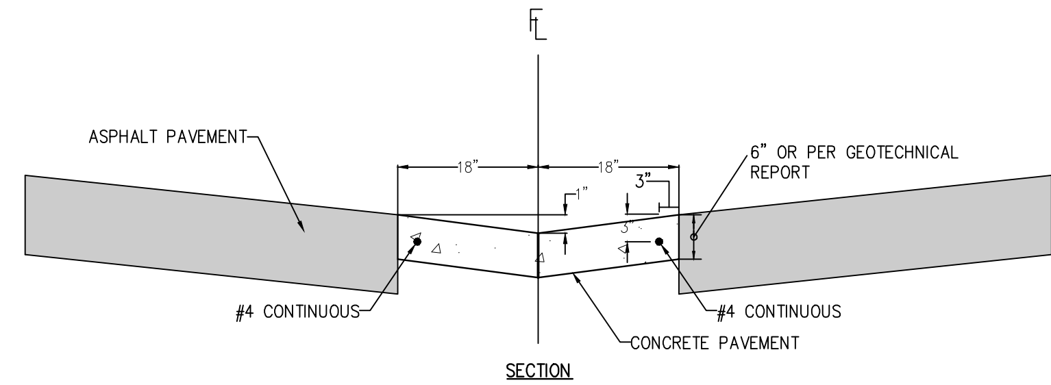
44 C-4.2 3" WIDE CONCRETE PAN DETAIL NOT TO SCALE
