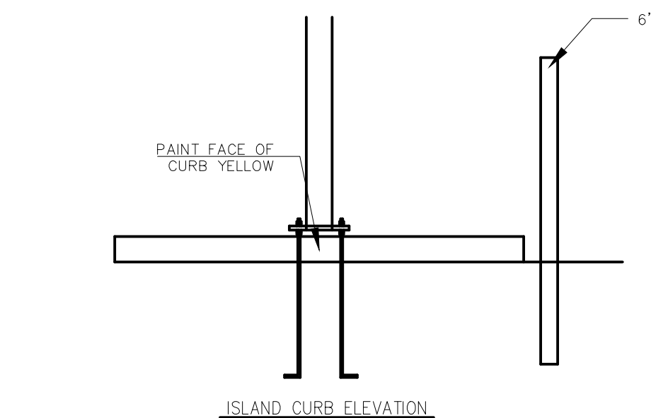
34 C-4.2 DRIVE THRU ORDER POINT ISLAND CURB NOT TO SCALE
