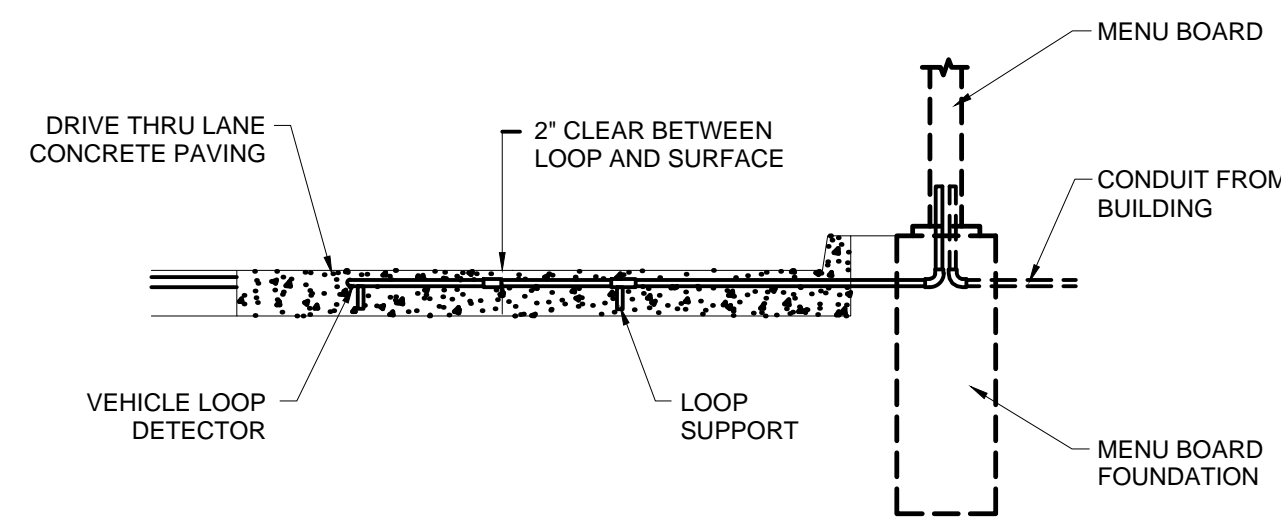
SECTION VIEW
