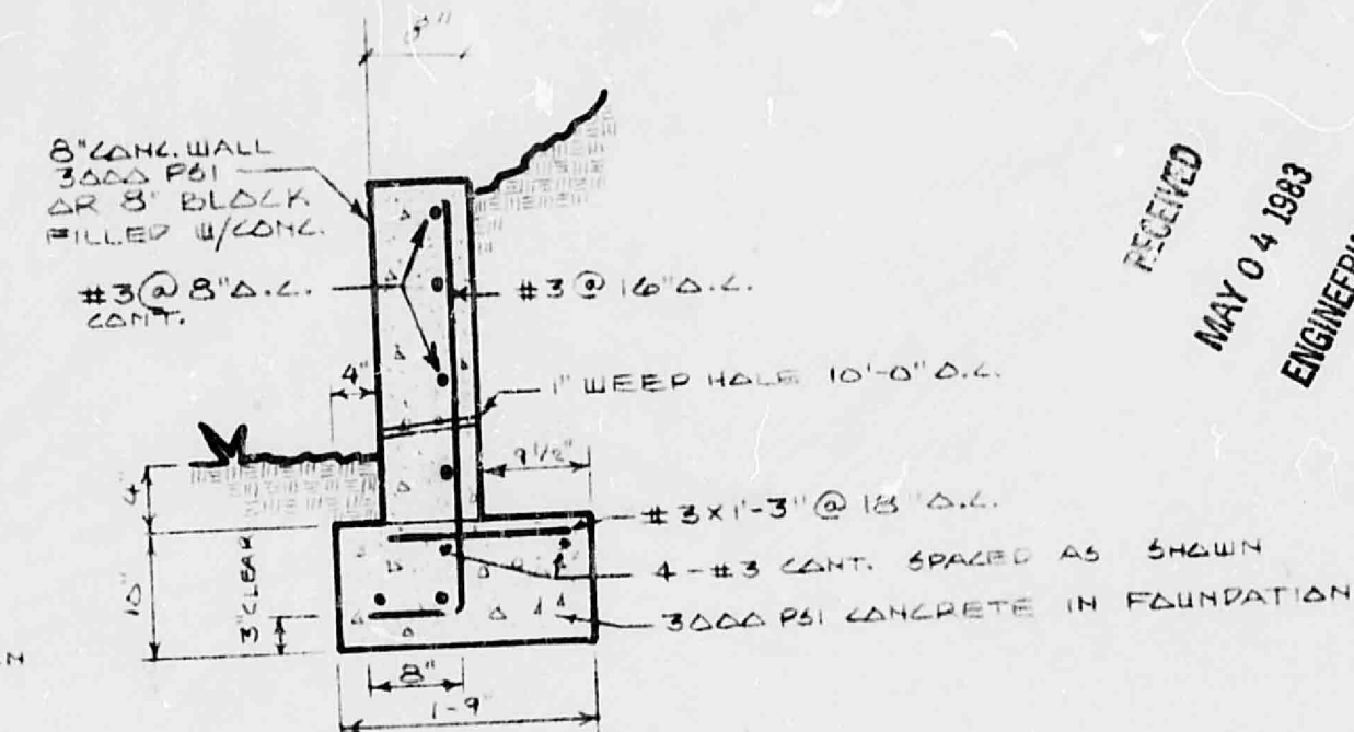
24" To 36" High Conc. Wall
