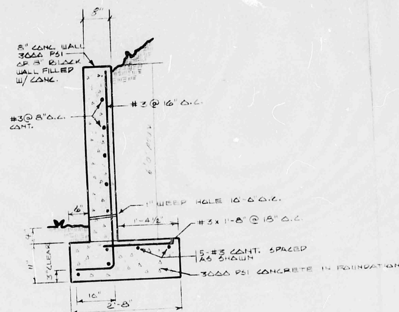
4' To 6' High Conc. Wall
