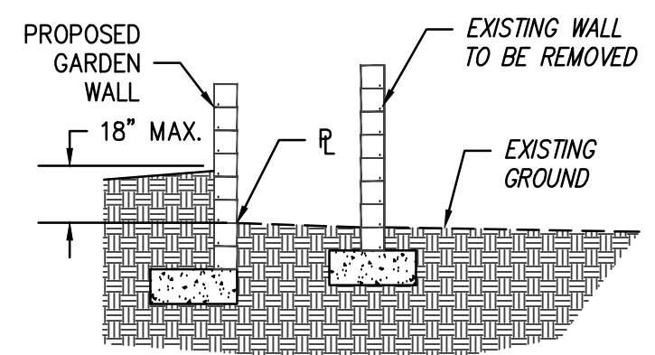
3 SECTION AT PROPERTY LINE Scale: 1:5
