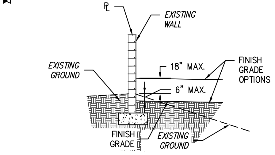
2 SECTION AT PROPERTY LINE Scale: 1:5
