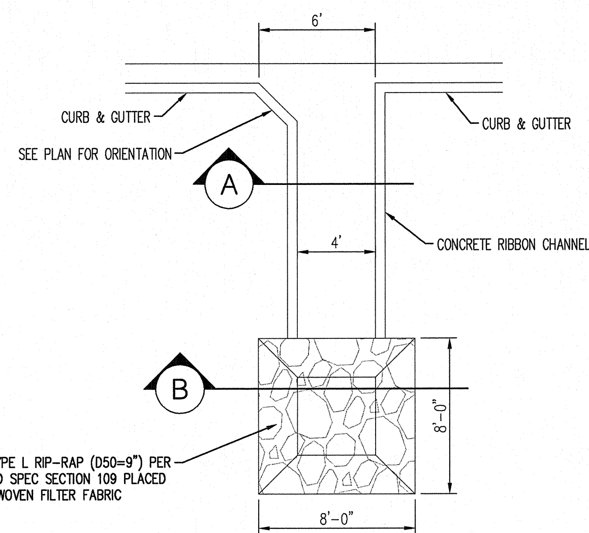
CONCRETE RUNDOWN & RIP-RAP PLUNGE POOL NOT TO SCALE
