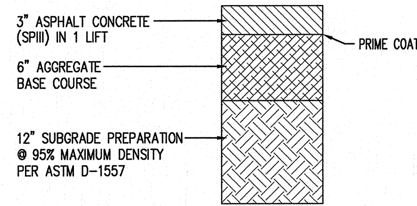
LIGHT DUTY PAVEMENT SECTION NOT TO SCALE
