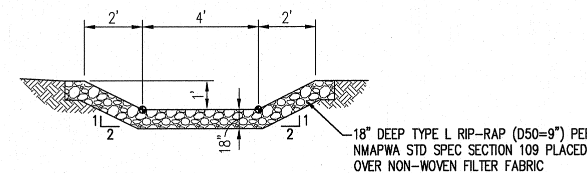
SECTION B NOT TO SCALE
