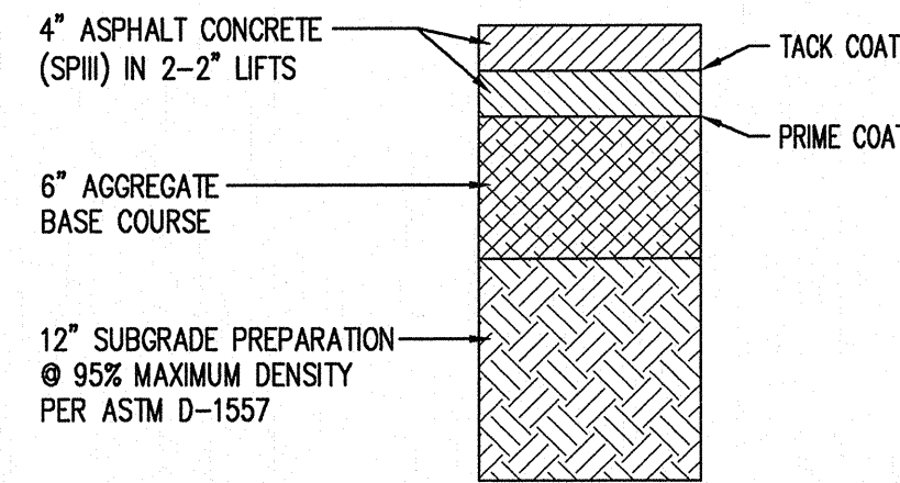
HEAVY DUTY PAVEMENT SECTION NOT TO SCALE
