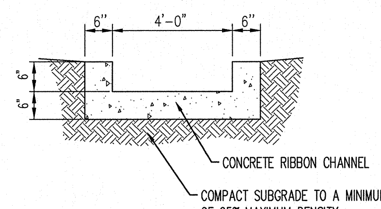
SECTION A NOT TO SCALE
