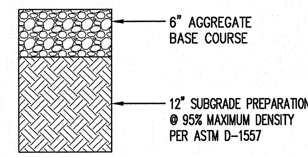
AGGREGATE BASE COURSE NOT TO SCALE
