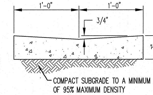
CONCRETE VALLEY GUTTER NOT TO SCALE
