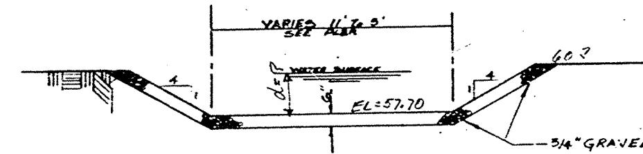
TYPICAL SECTION PONDING AREA
