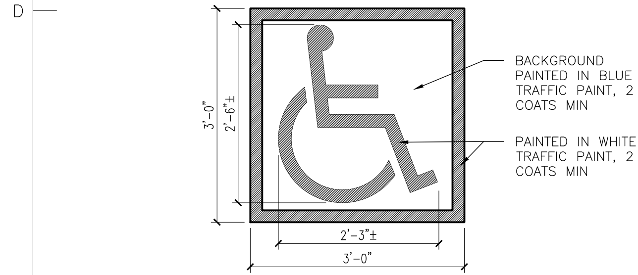
C1 ACCESSIBLE PARKING PAVEMENT MARKING SCALE: 3/4" = 1'-0"
