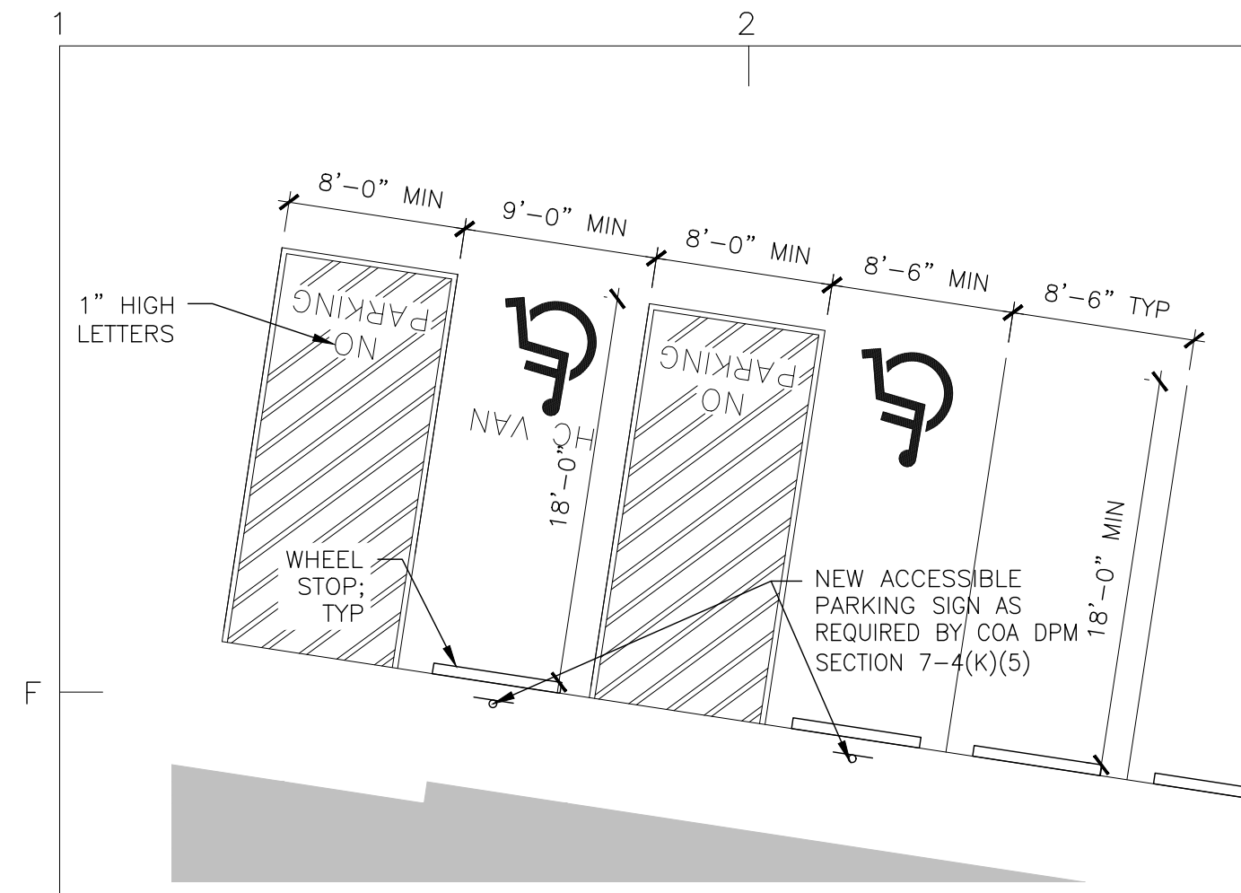
E1 ACCESSIBLE PARKING SCALE: 1/2" = 1'-0"
