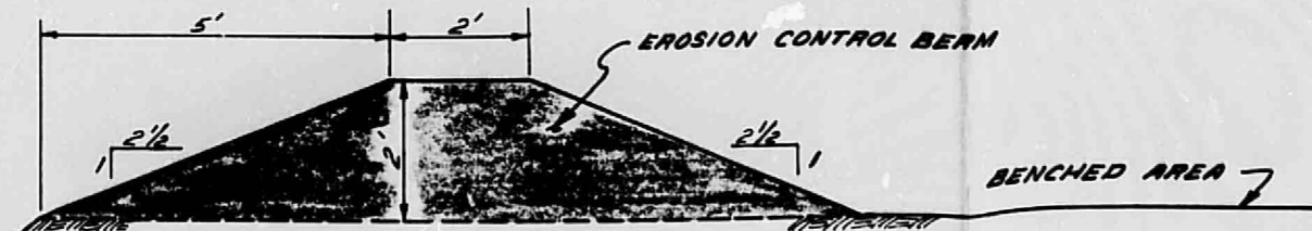
TYPICAL EROSION CONTROL BERM SECTION NO SCALE
