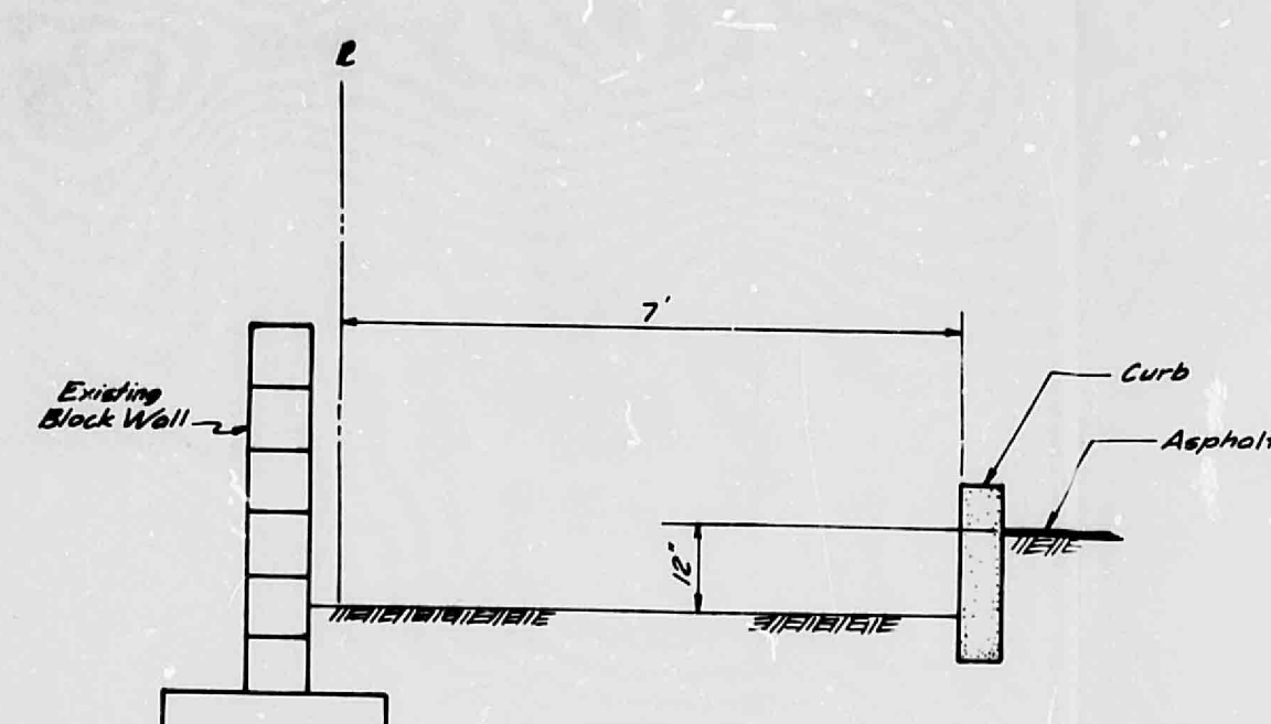
SECTION 1 SCALE 1" = 2'
