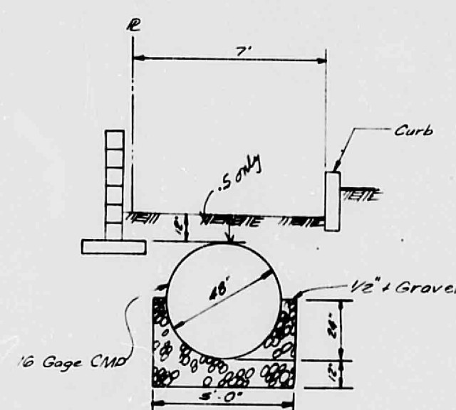
SECTION 3 SCALE 1" = 4'
