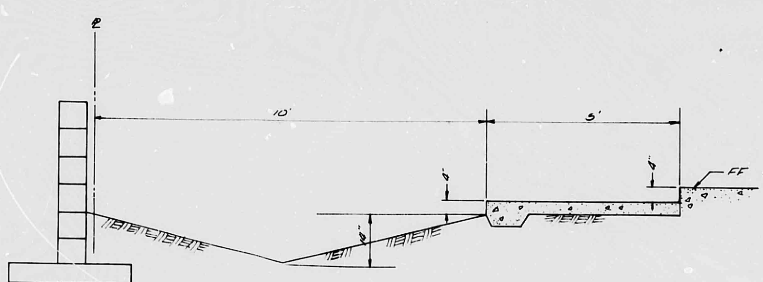
SECTION 2 SCALE 1" = 2'
