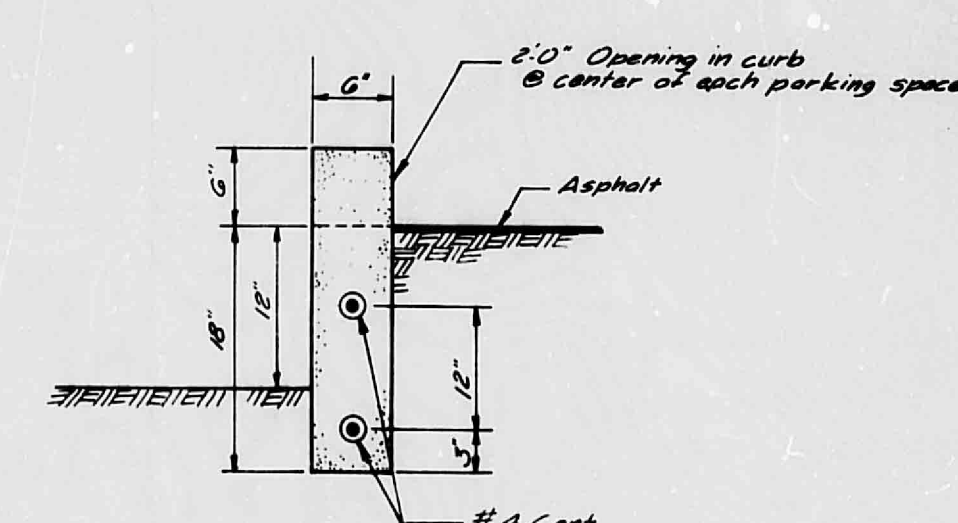
TYPICAL CURB SCALE 1" = 1'
