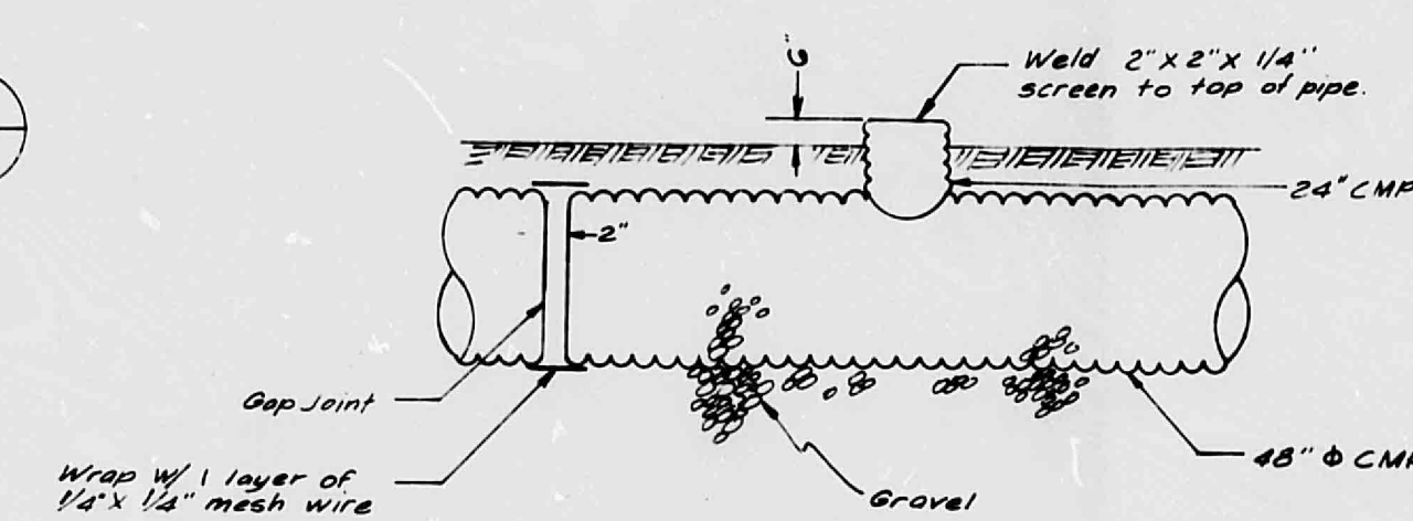
SECTION 4 NO SCALE
