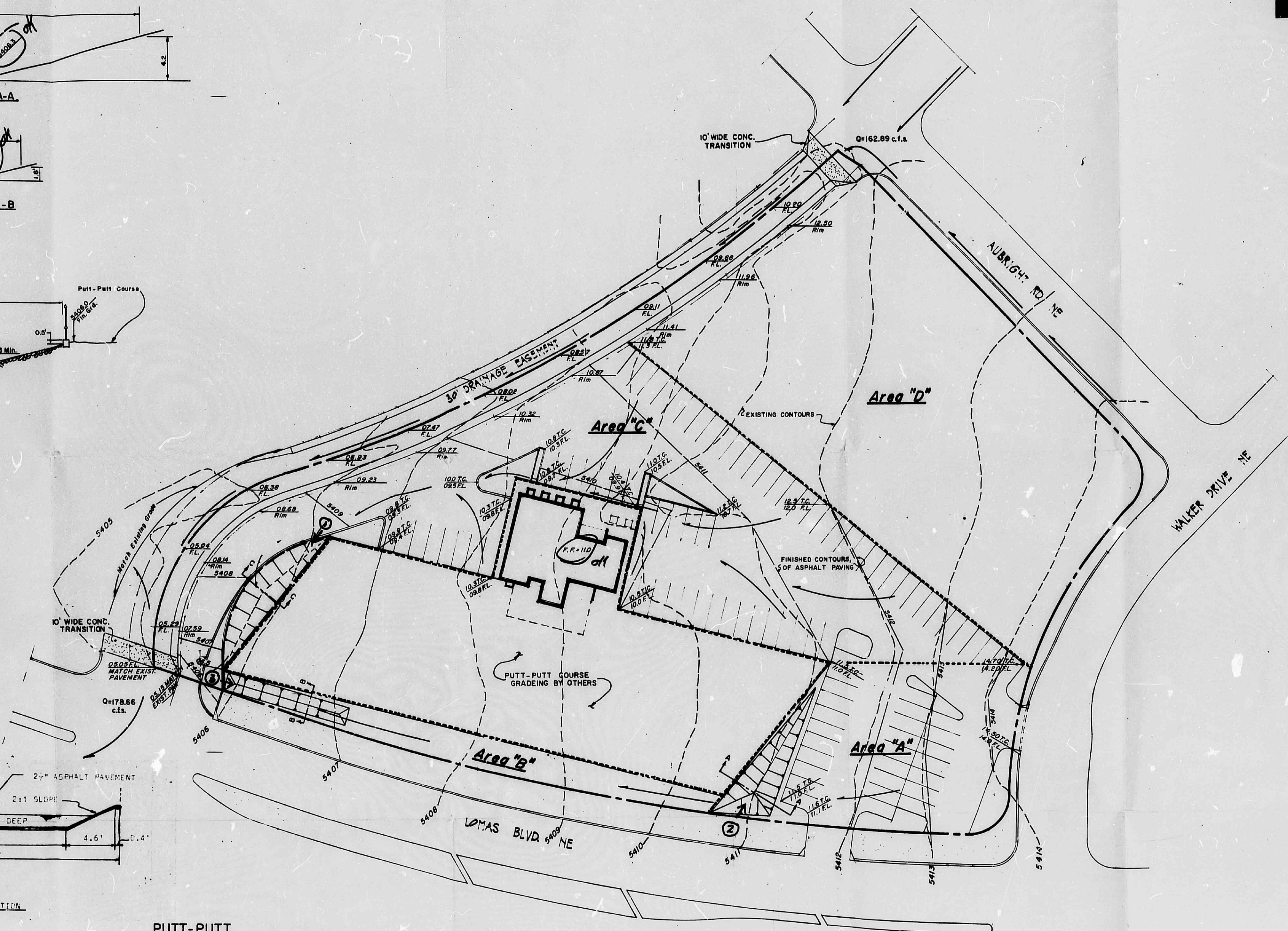
PUTT-PUTT DRAINAGE & GRADING PLAN
