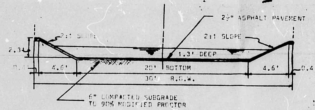
DRAINAGE R.E.M. CHANNEL SECTION
