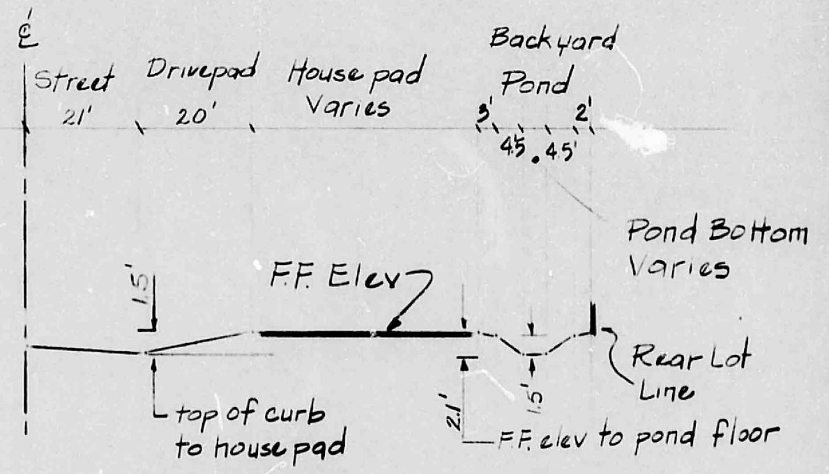
TYPICAL LOT SECTION No Scale
