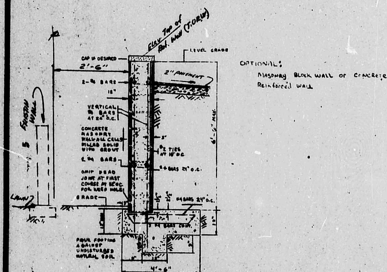
SECTION 4 - RETAINING WALL SCALE 1" = 1'-0"
