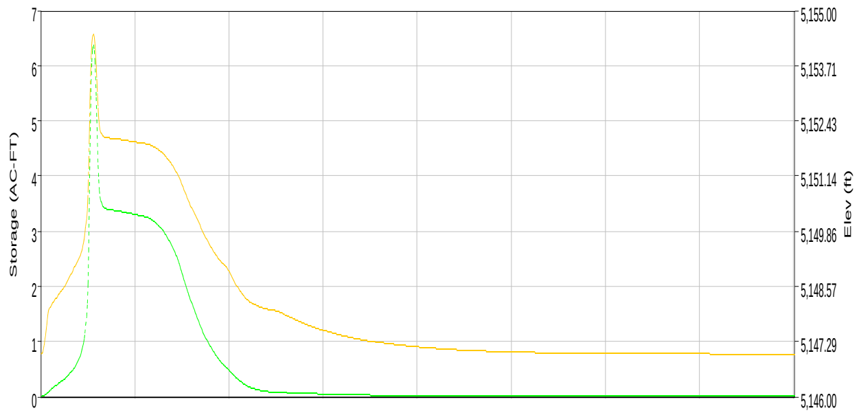
Reservoir "POND 4" Results for Run "DEVEX_1"
