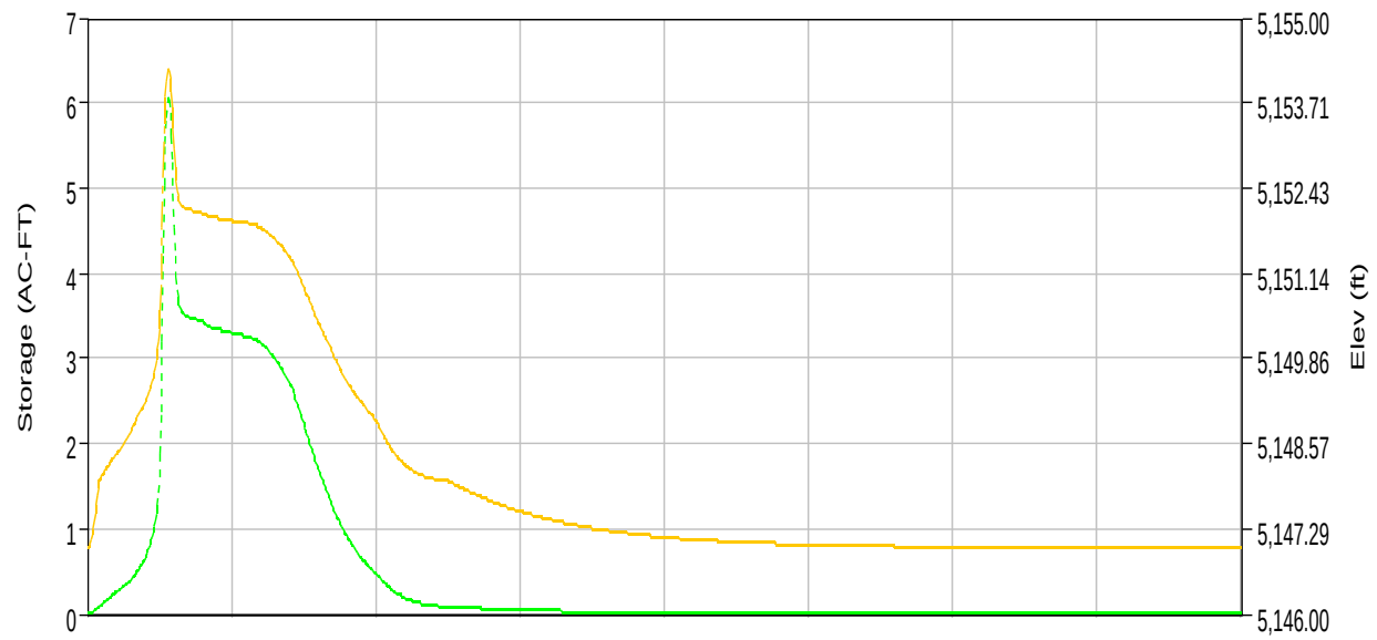
Reservoir "POND 4" Results for Run "DEVEX_2"
