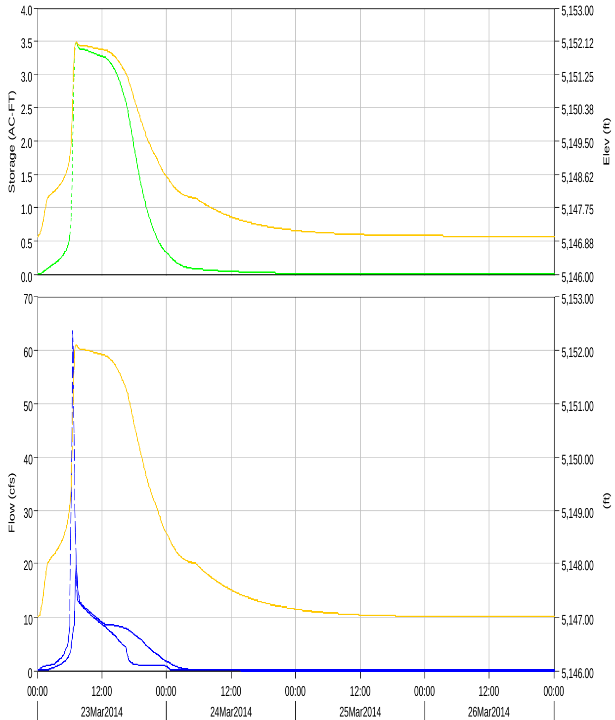
Reservoir "POND 4" Results for Run "Existing"
