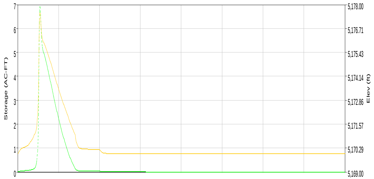
Reservoir "POND 6" Results for Run "DEVEX_2"
