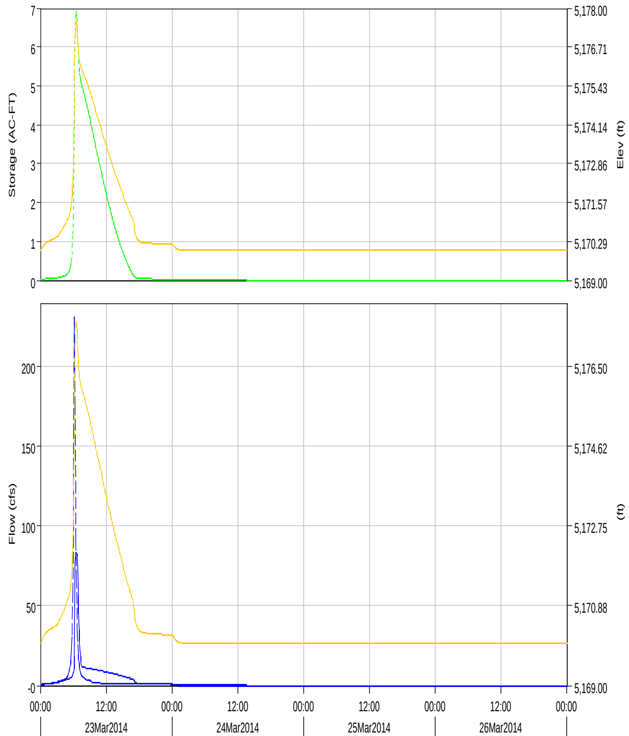
Reservoir "POND 6" Results for Run "DEVEX_OPTION1"
