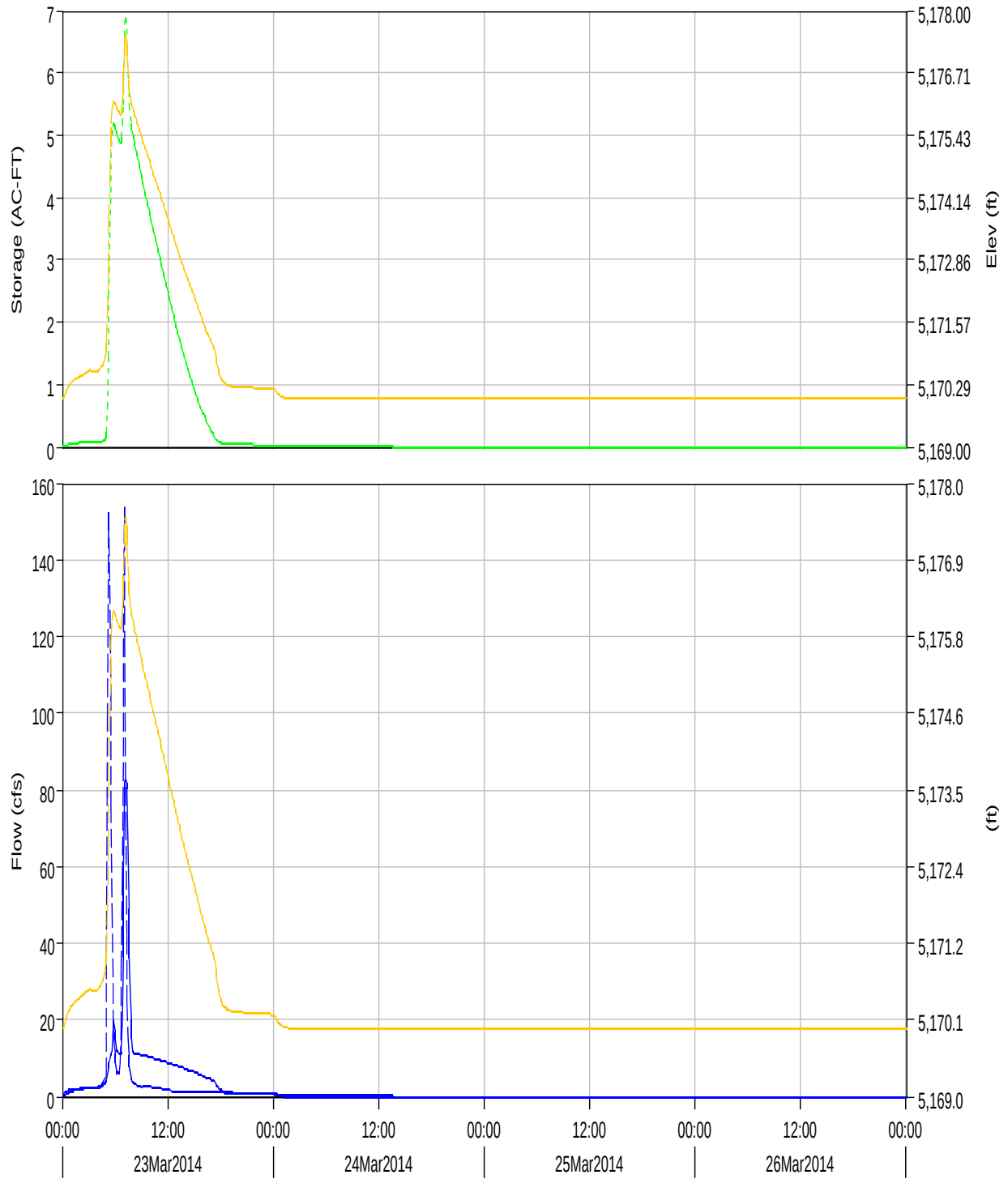
Reservoir "POND 6" Results for Run "DEVEX_SMITH"
