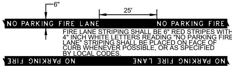
FIRE LANE MARKING
