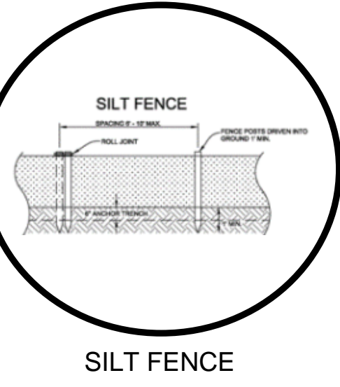
SILT FENCE
