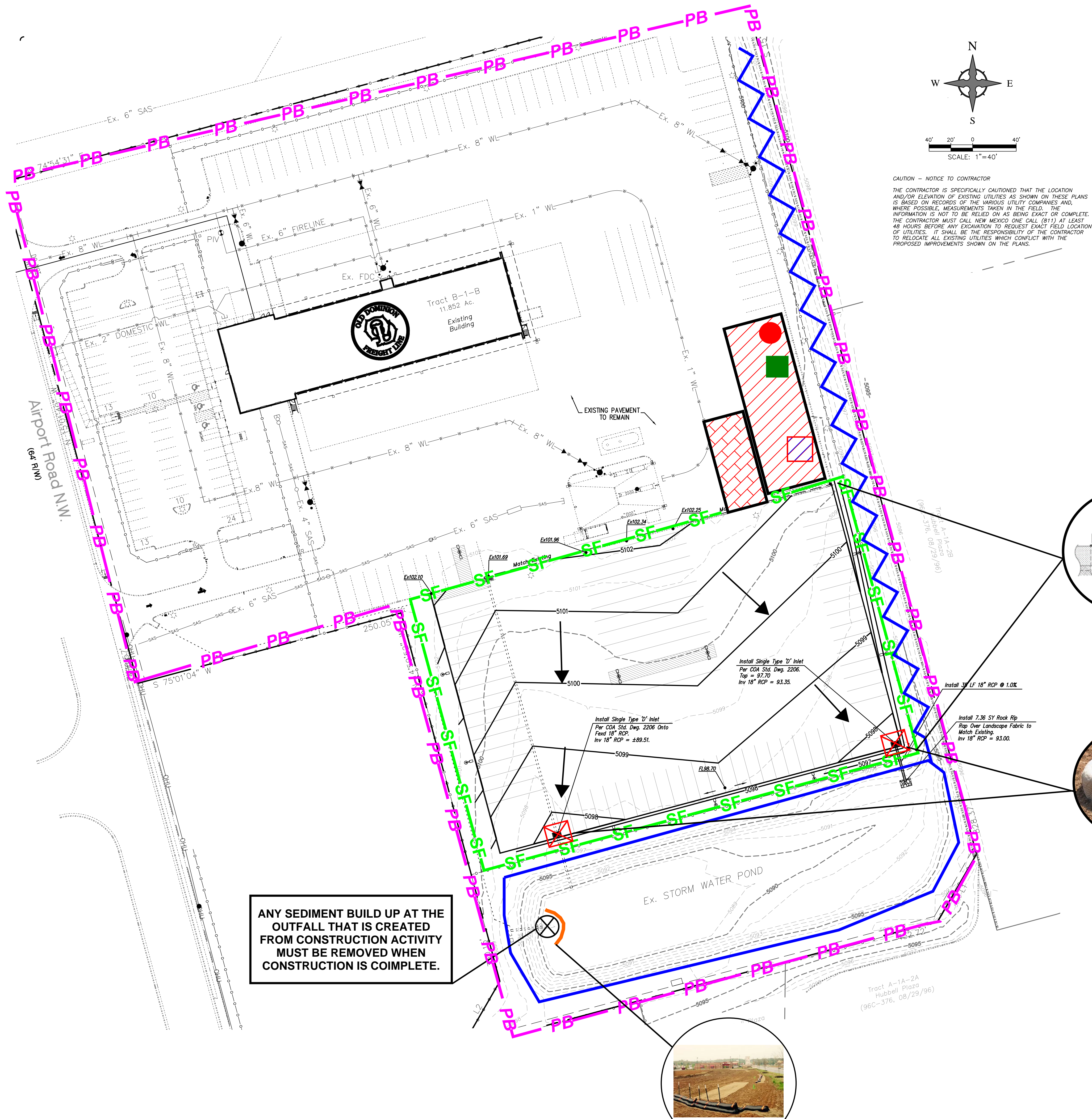
INLET PROTECTION
