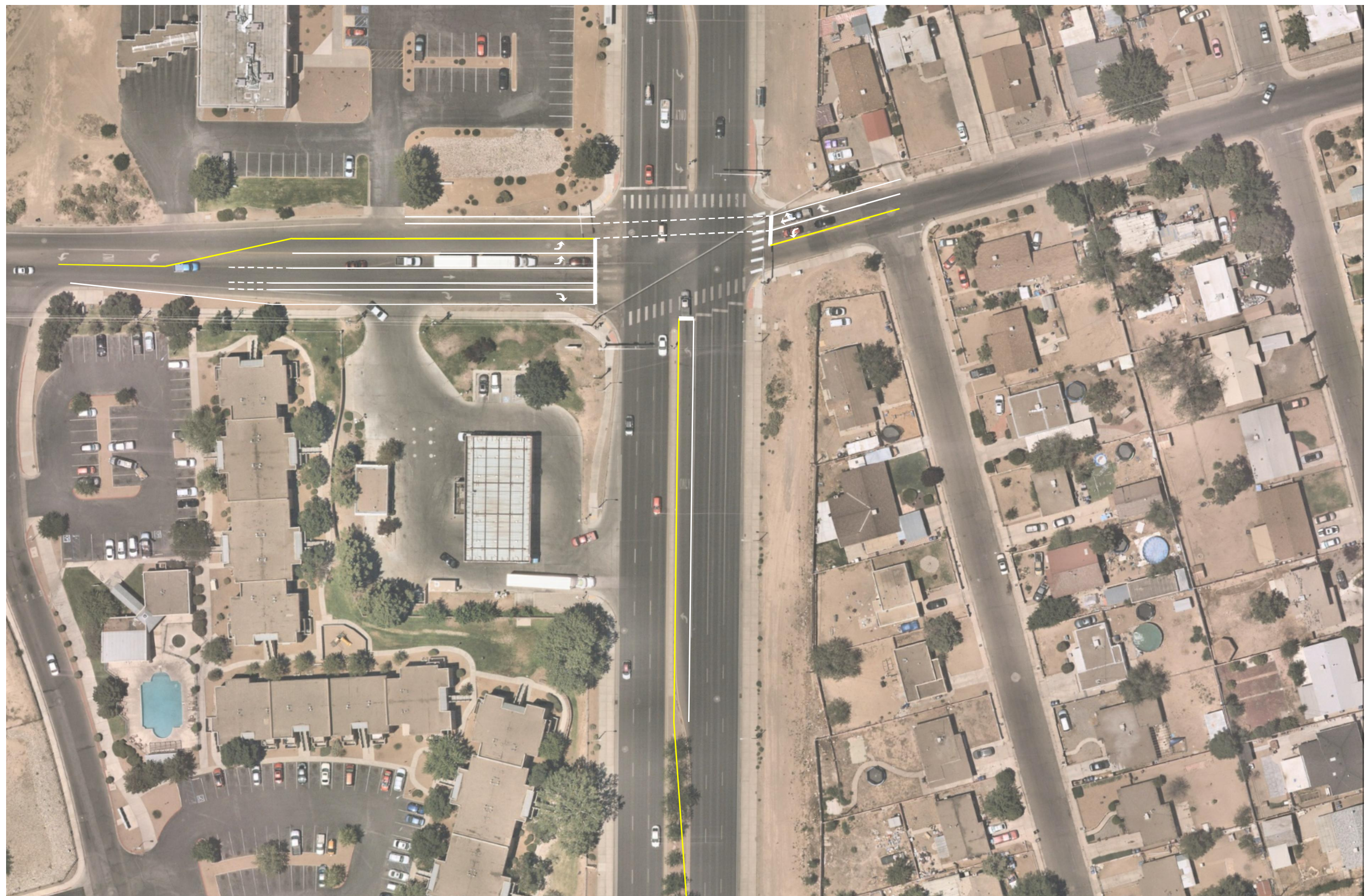
ABB EXPANSION ALBUQUERQUE, NEW MEXICO BLUEWATER RD & COORS BLVD PROPOSED STRIPING
