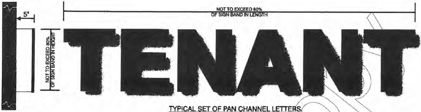
SIDE VIEW
