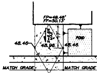
DRIVEPAD ELEVATIONS
