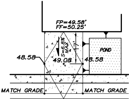
DRIVEPAD ELEVATIONS
