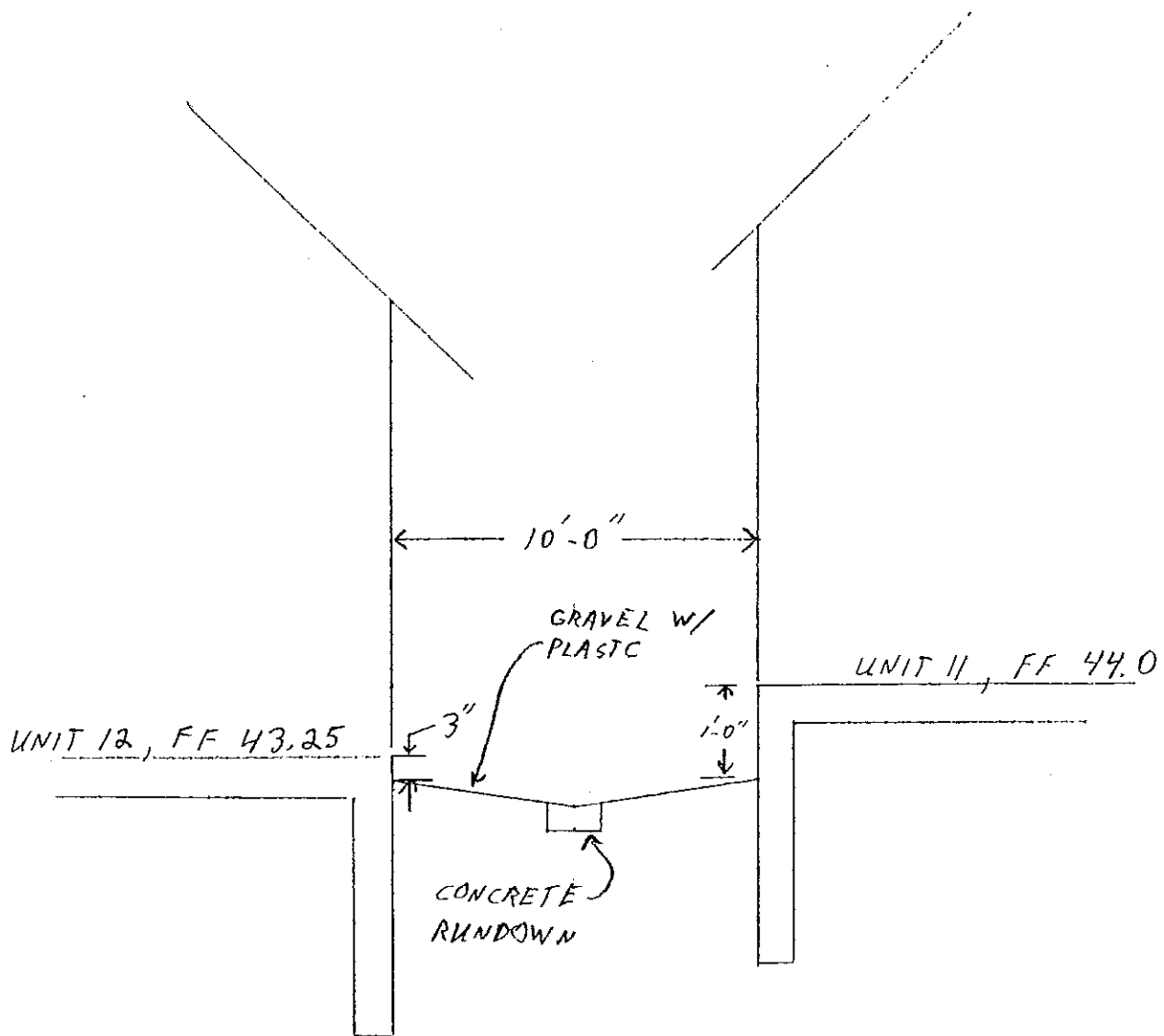
ELEVATION (SECTION A-A)
