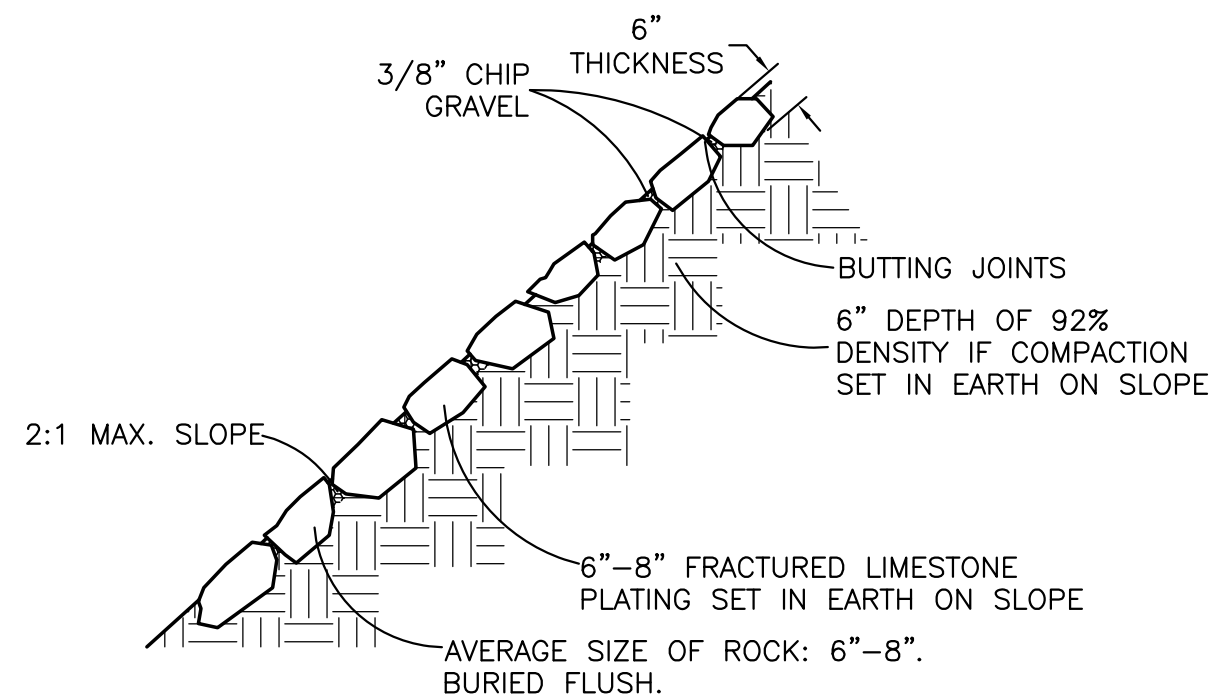
ROCK PLATING DETAIL NTS
