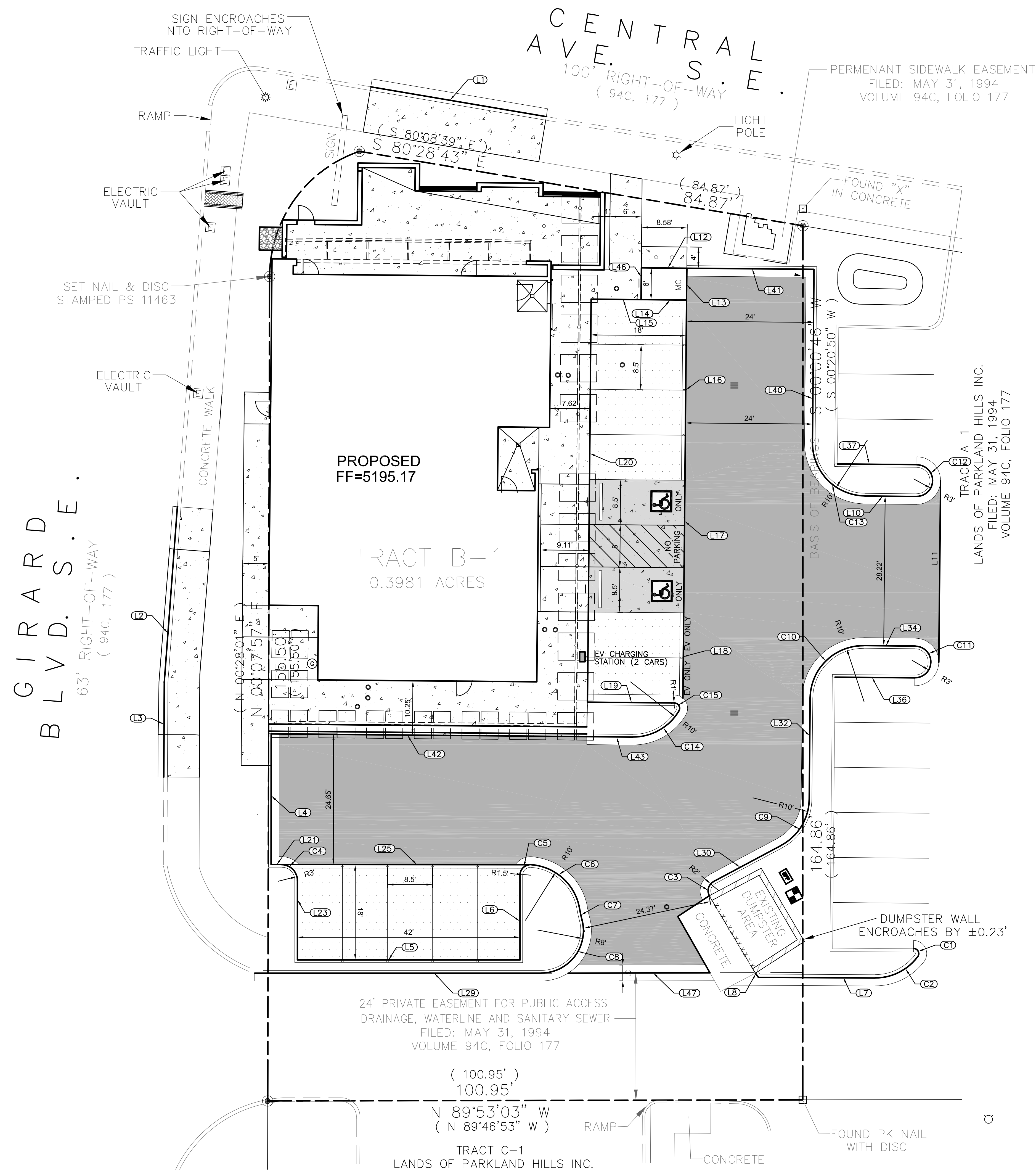
A1 TRAFFIC CIRCULATION LAYOUT 1"=10'-0"
