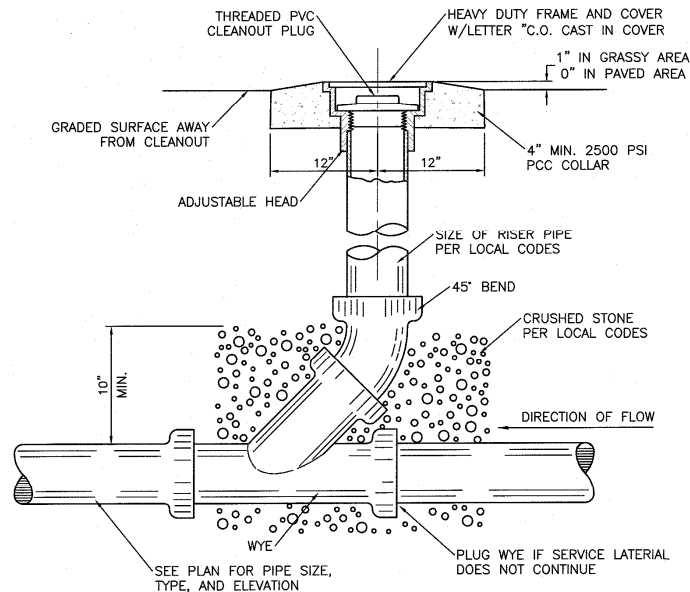
SANITARY SEWER CLEAN-OUT NTS
