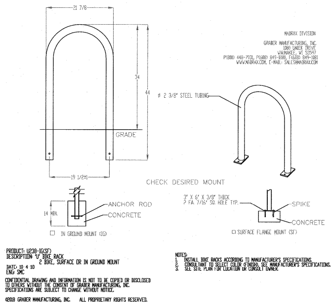
BIKE RACK DETAIL SCALE: NONE
