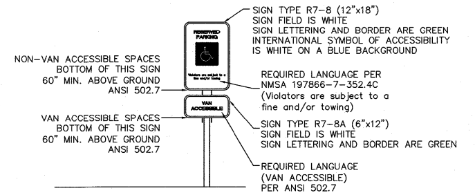
ACCESSIBLE PARKING SIGN NTS
