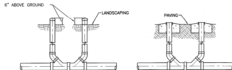
SANITARY SEWER CLEAN-OUT NTS
