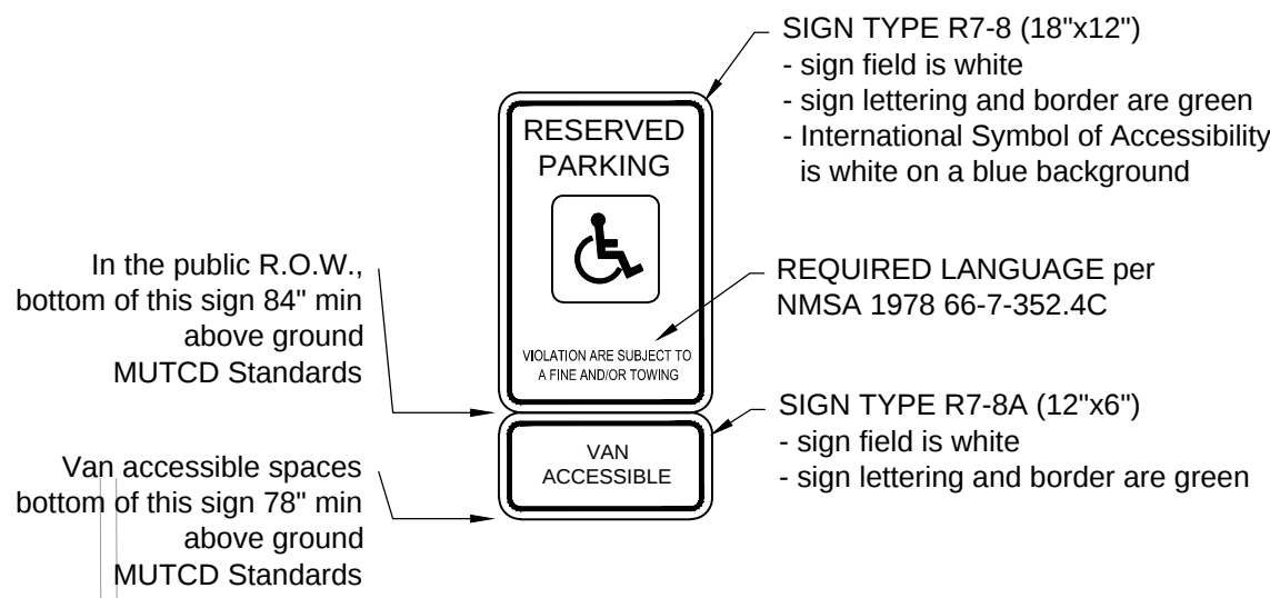
ADA SIGN FACE DETAIL
