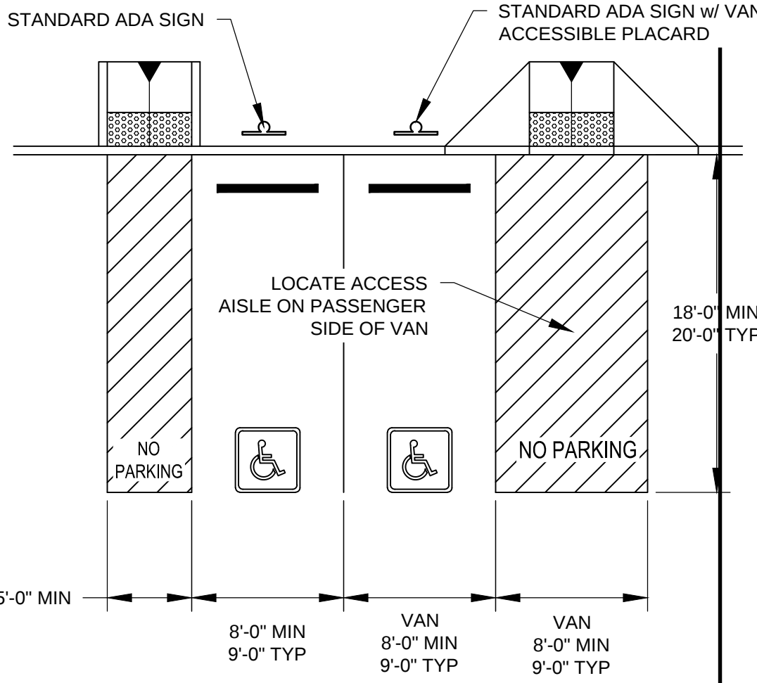
ACCESSIBLE PARKING DETAIL
