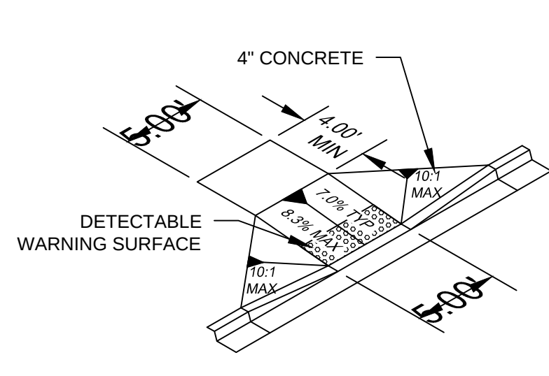
ADA RAMP TYPE "A"
