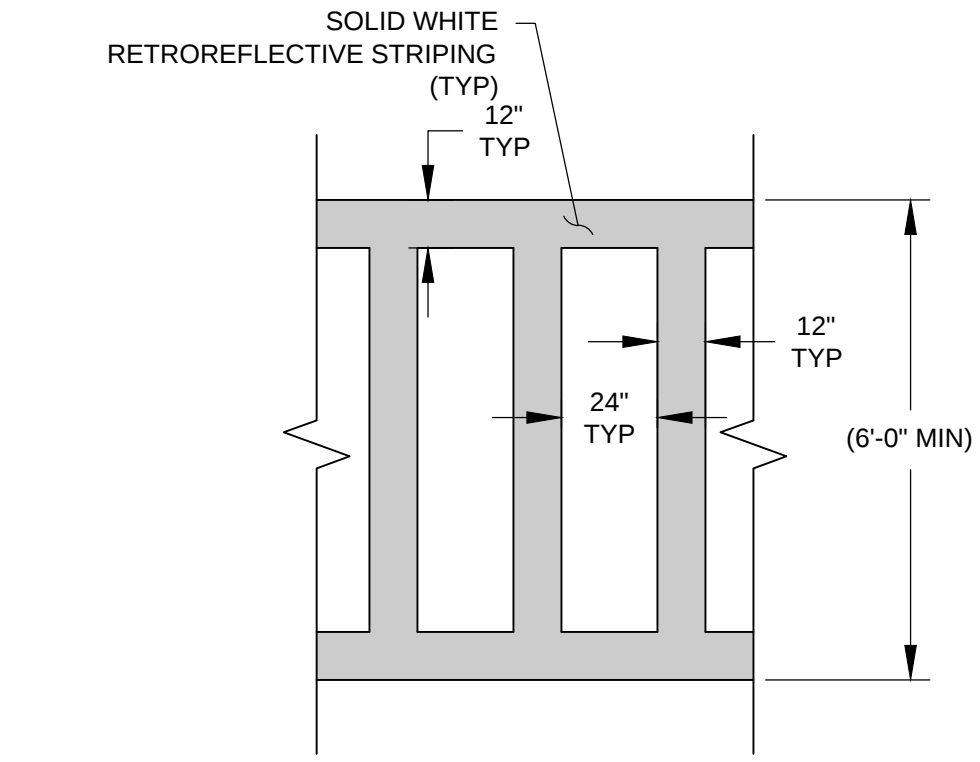
CROSSWALK STRIPING DETAIL
