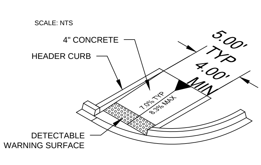
ADA RAMP TYPE "B"
