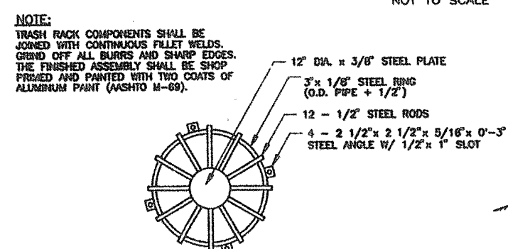
TRASH RACK - PLAN VIEW NOT TO SCALE
