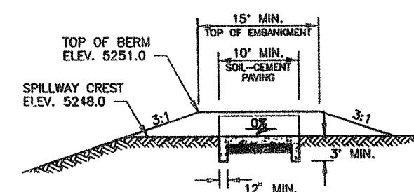
SPILLWAY STRUCTURE - SECTION E-E NOT TO SCALE
