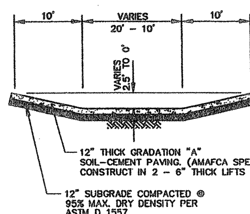
RUNDOWN STRUCTURE - SECTION B-B NOT TO SCALE
