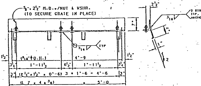
SEAT ANGLE DETAILS
