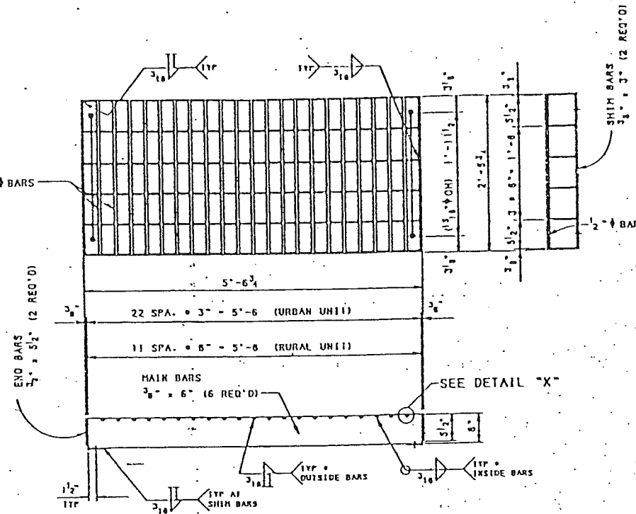
GRATE DETAILS (2 REQUIRED)
