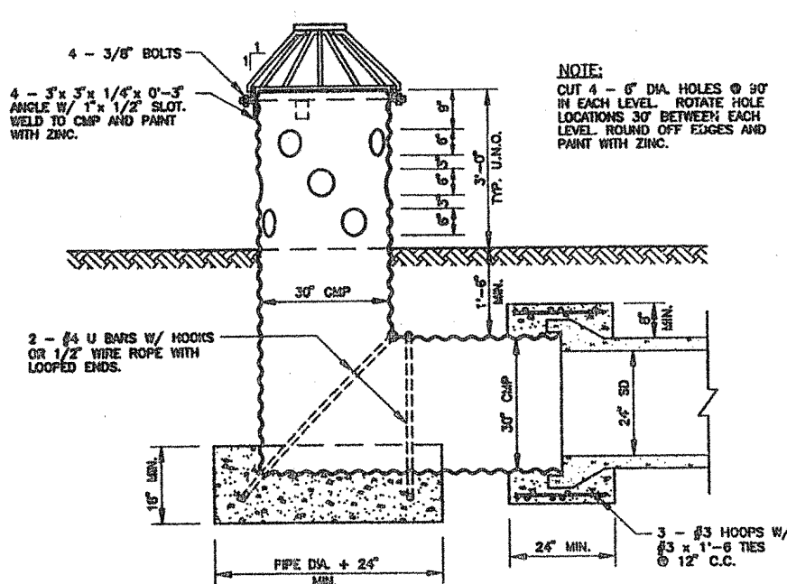
CMP INLET STRUCTURE NOT TO SCALE
