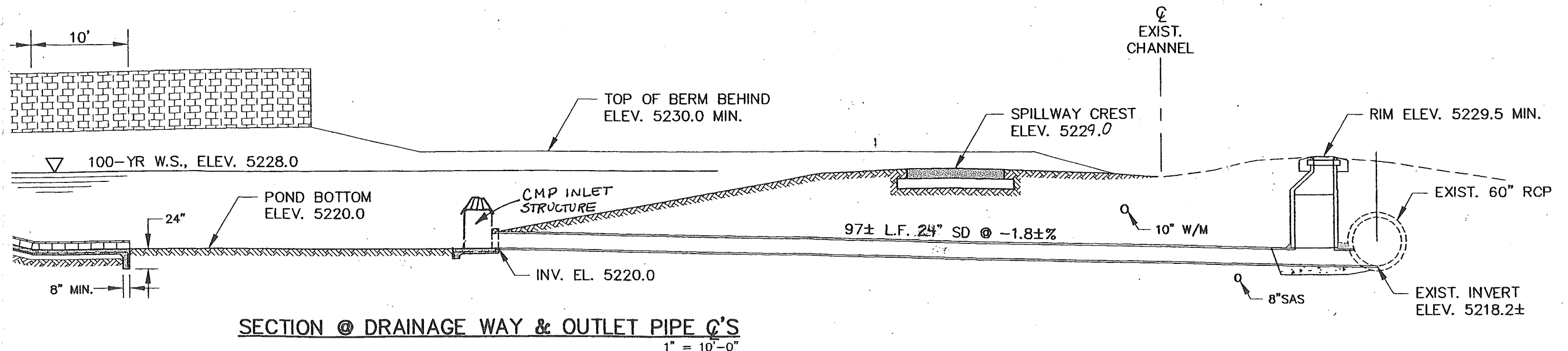
Figure 6 Onsite Detention Pond Outfall Structure
