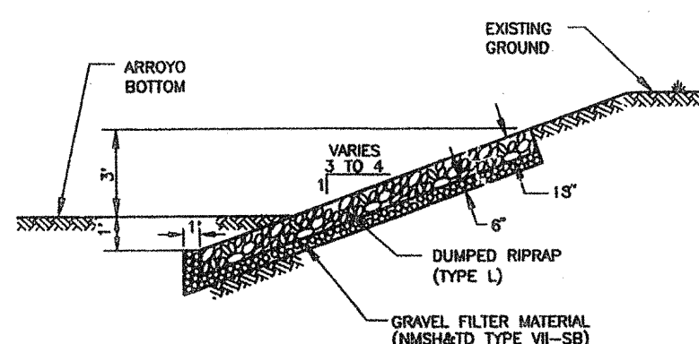
TYPICAL RIPRAP SLOPE PROTECTION - SECTION D-D NOT TO SCALE
