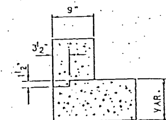
CONST. JOINT DETAIL
