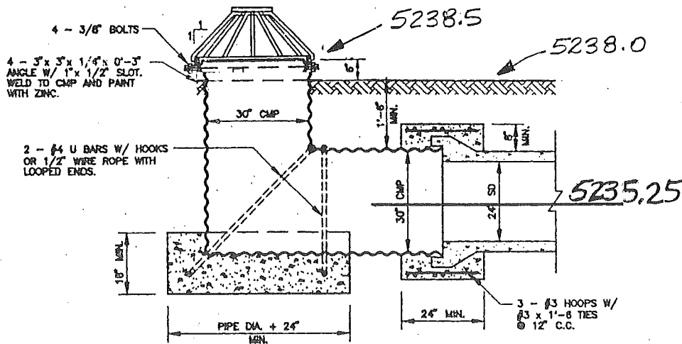
CMP INLET STRUCTURE NOT TO SCALE
