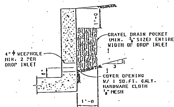
WEEP HOLE DETAIL
