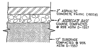
2 C7 LIGHT TRAFFIC PAVING SECTION N.T.S.
