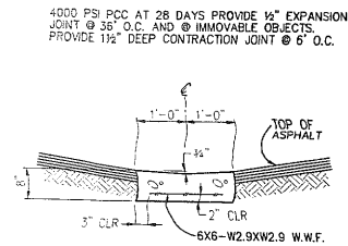
3 C7 CONCRETE VALLEY CUTTER 1/4"=1'-0"
