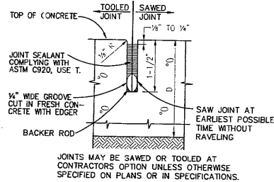
5 C7 CONTRACTION JOINT (CJ) N.T.S.
