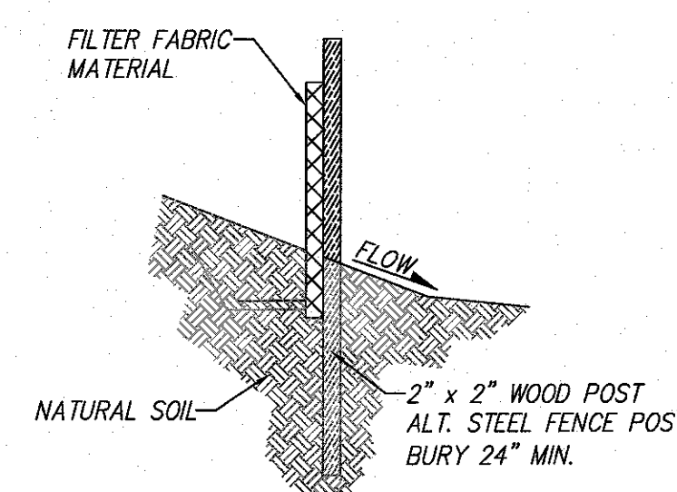
SILT FENCE FOR SEDIMENT CONTROL
