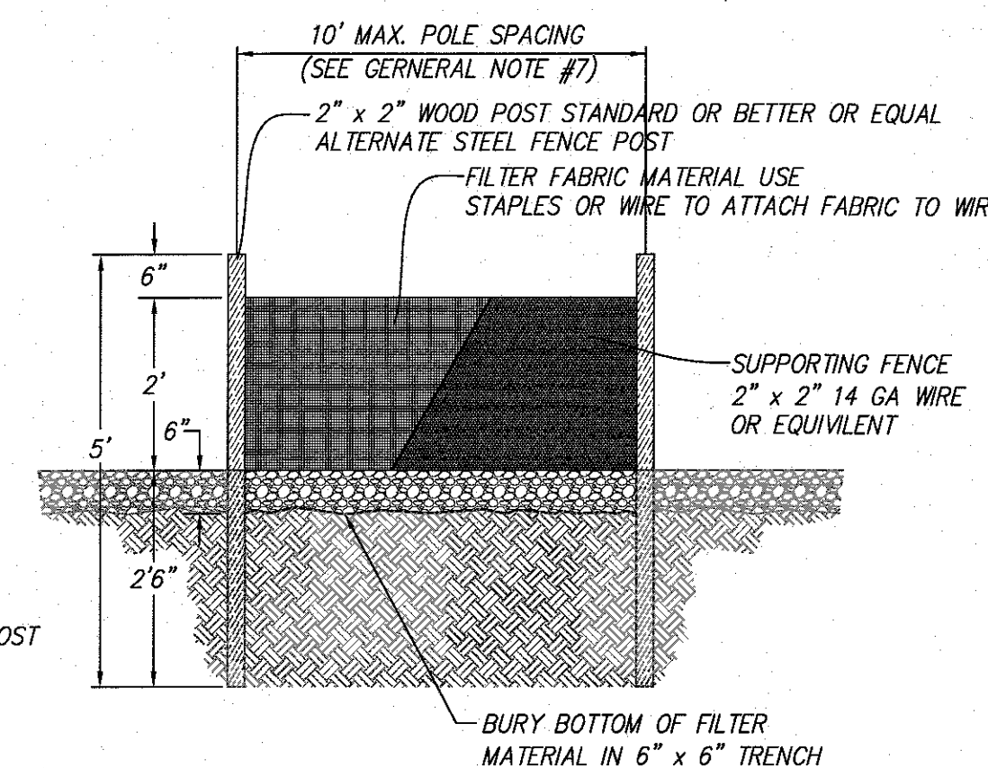
SILT FENCE FOR SEDIMENT CONTROL
