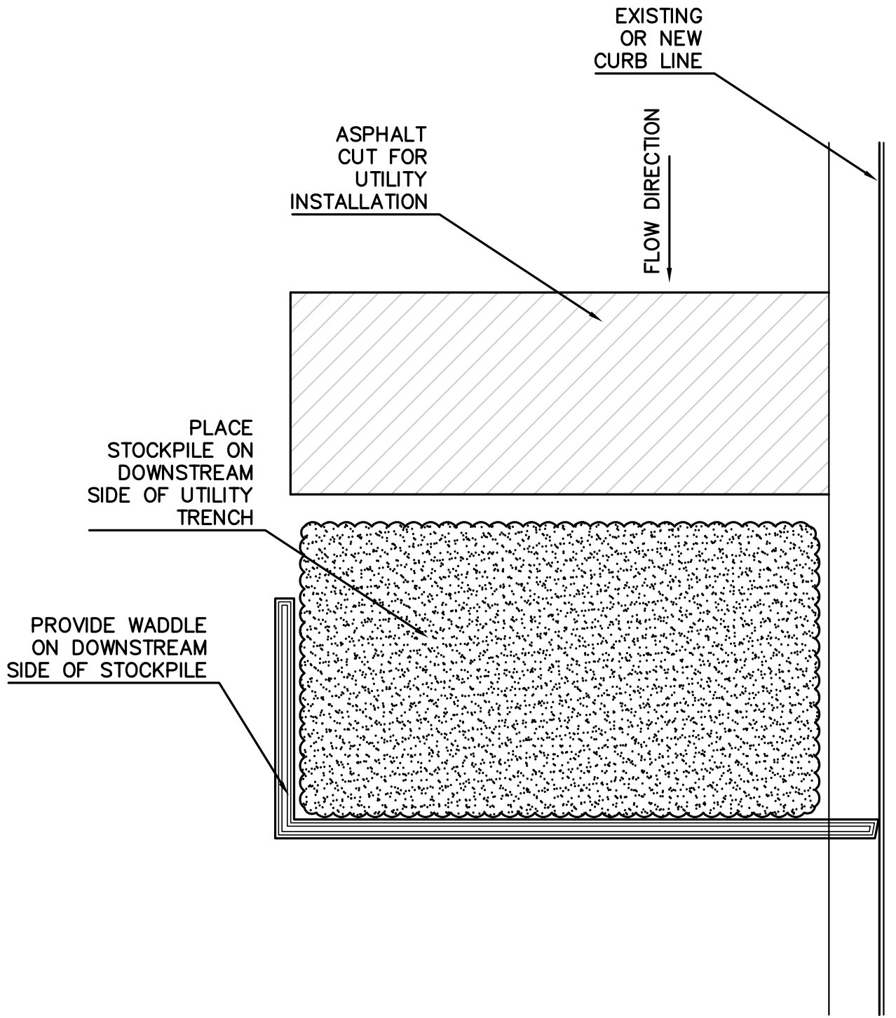
TYPICAL UTILITY CUT DETAIL NOT TO SCALE
