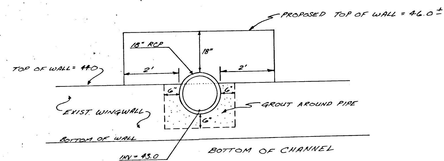
HEADWALL DETAIL AT OUTLET 1"=2'
