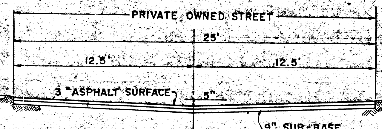
SECTION A-A NOTE: SUB-BASE COMPACTED TO 95% PROCTOR
