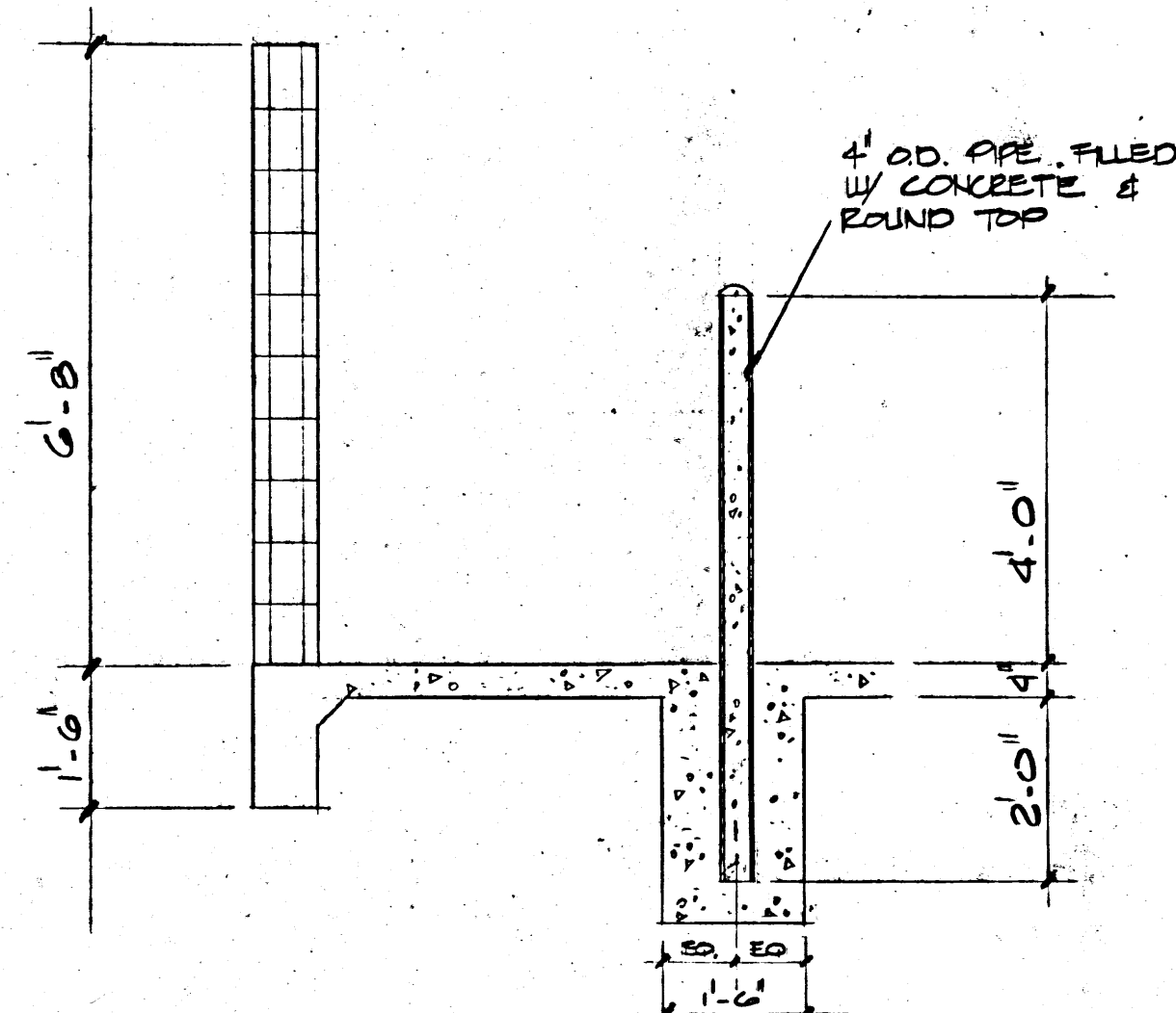
2 SCREEN WALL SECT. 1/2" = 1'-0"
