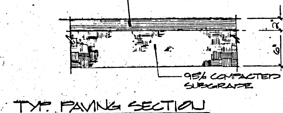
5 PAVING DETAILS NTS.
