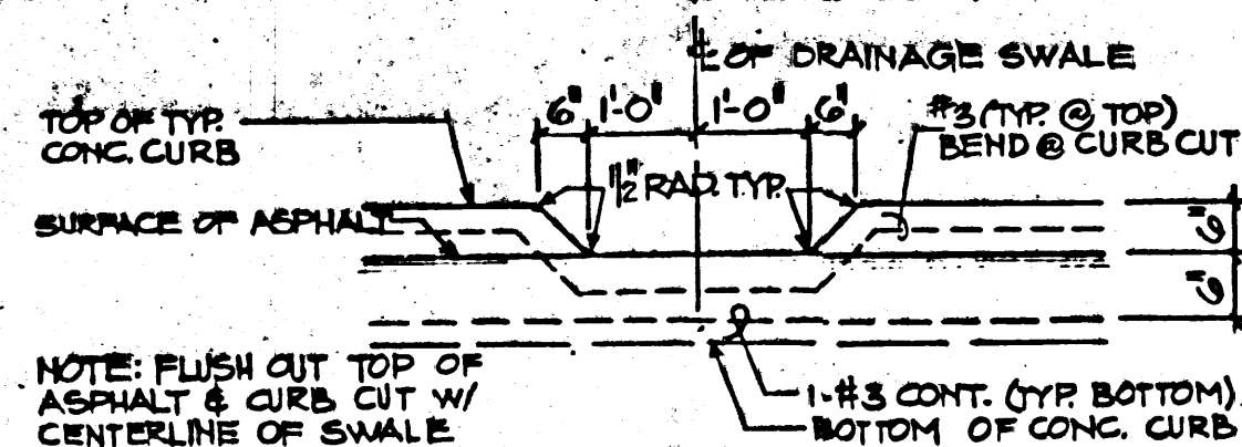
5A CURB CUT AT DRNG. SWALE NTS.
