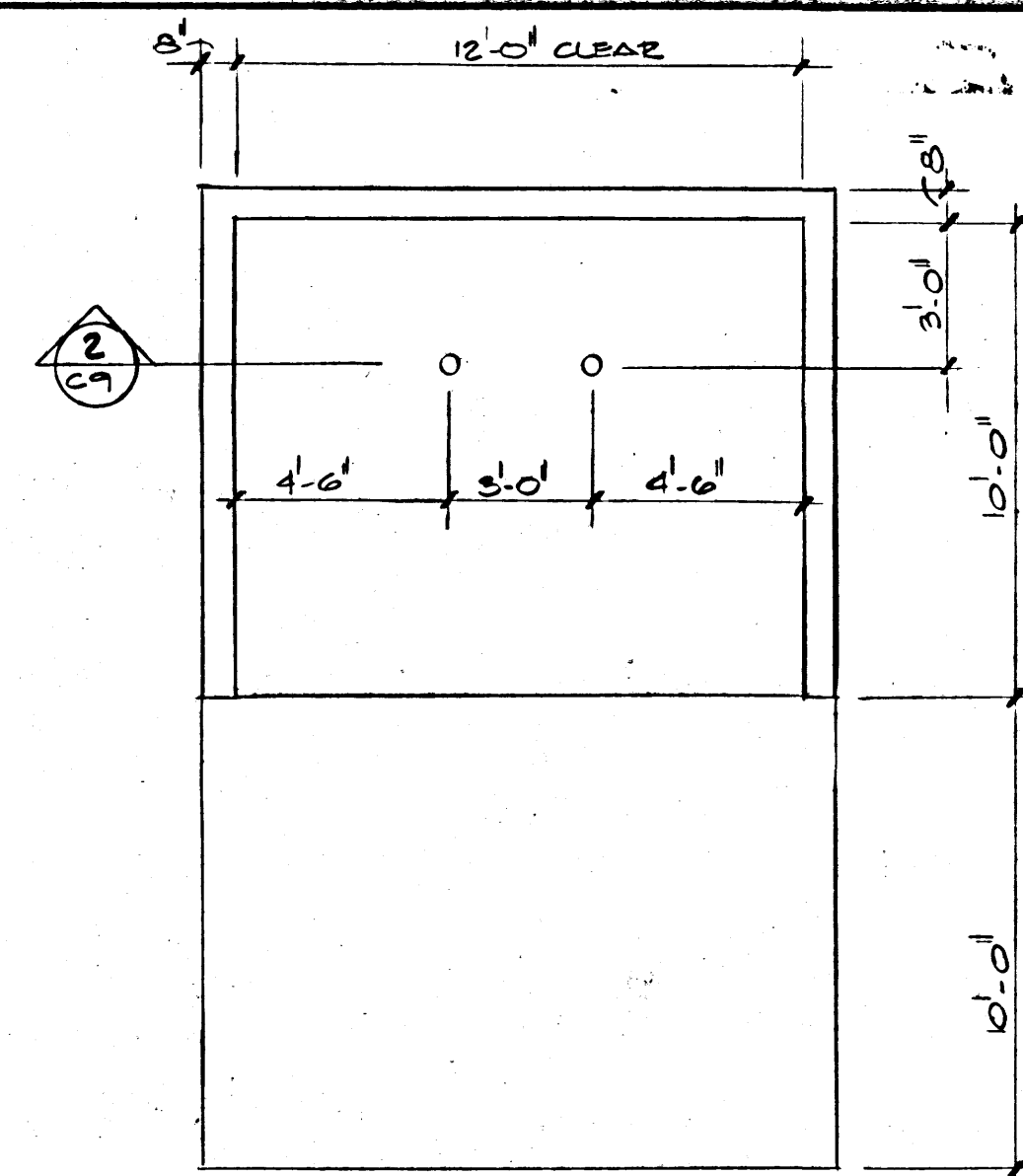
1 DUMPSTER SCREEN WALL 1/2" = 1'-0"
