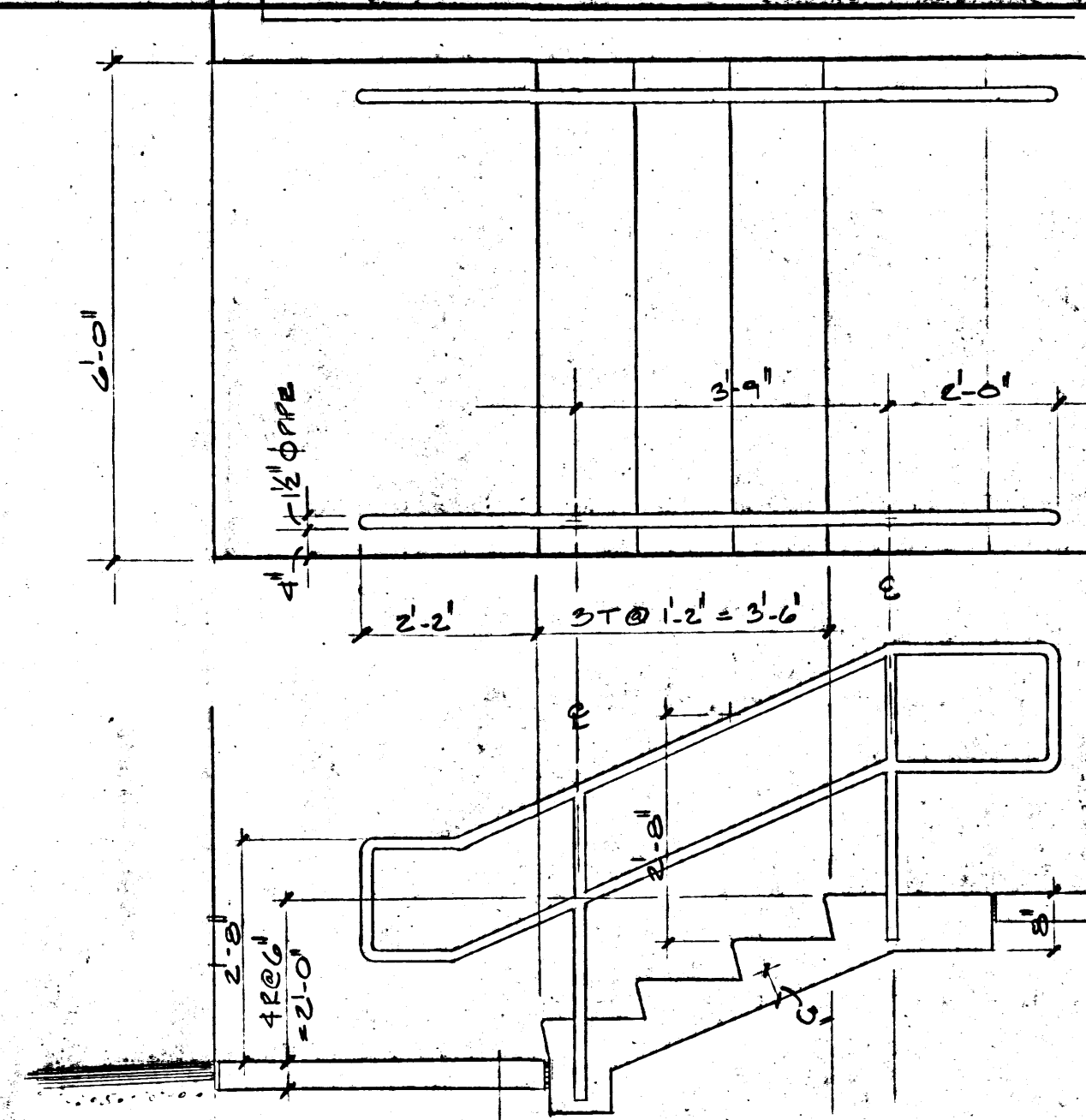
3 EXTERIOR STAIRS 1/2" = 1'-0"
