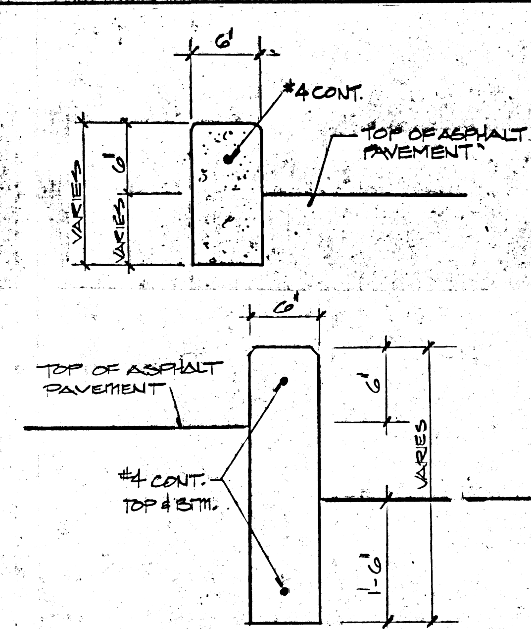
4 CURB DETAILS NTS.
