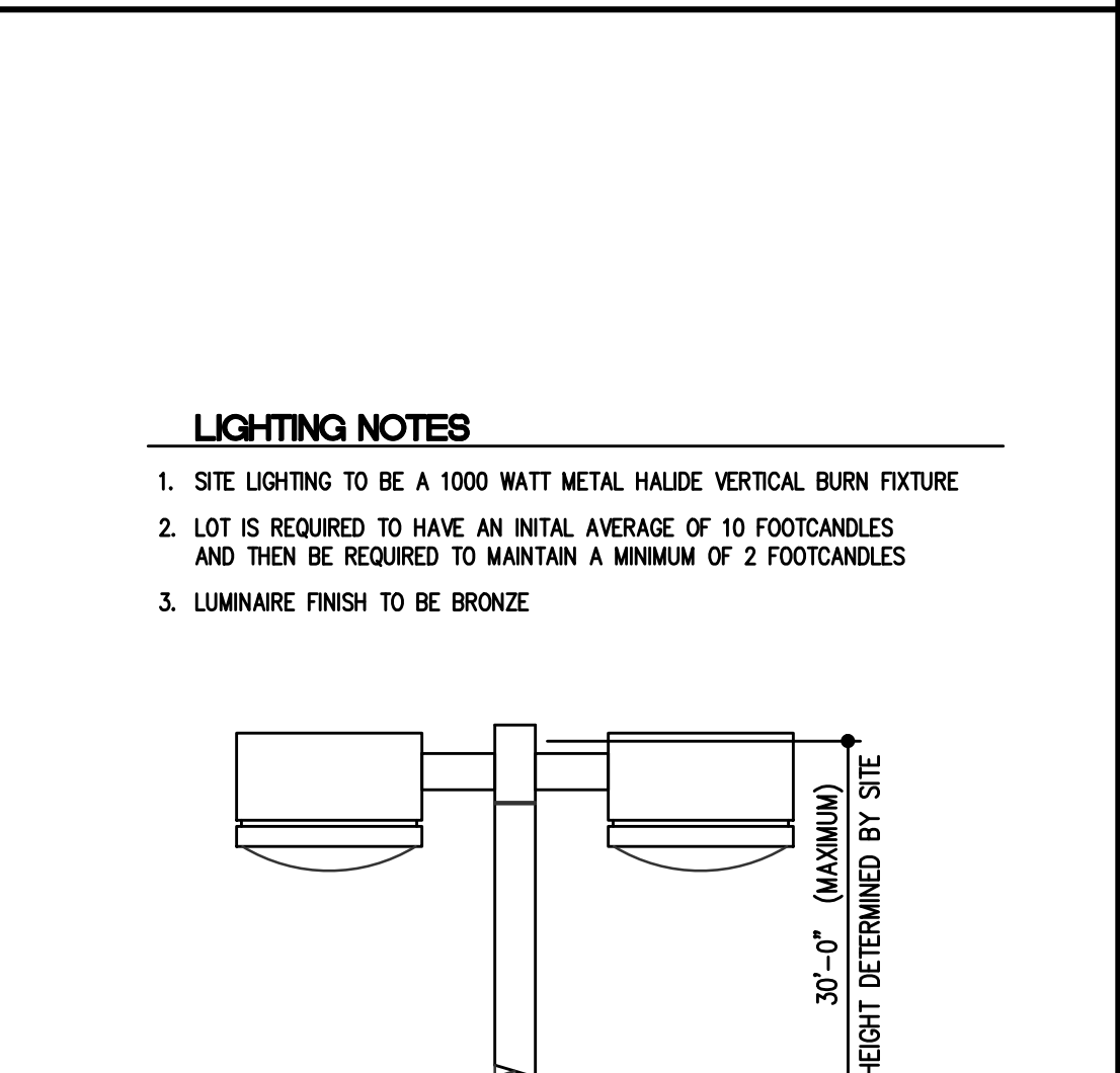
E EXTERIOR POLE LIGHTS AC2 NOT TO SCALE
