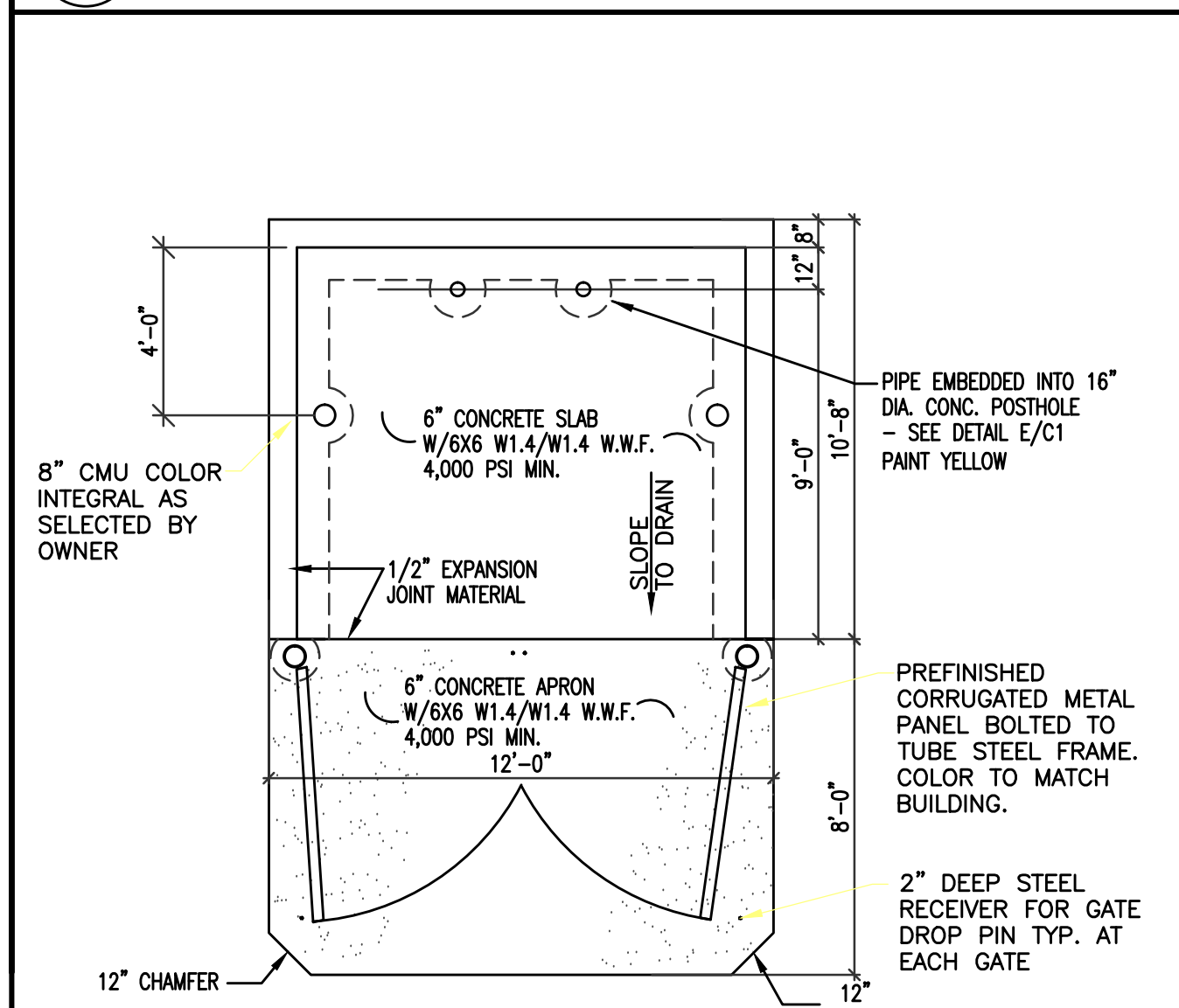
A TRASH ENCLOSURE AC2 NOT TO SCALE
