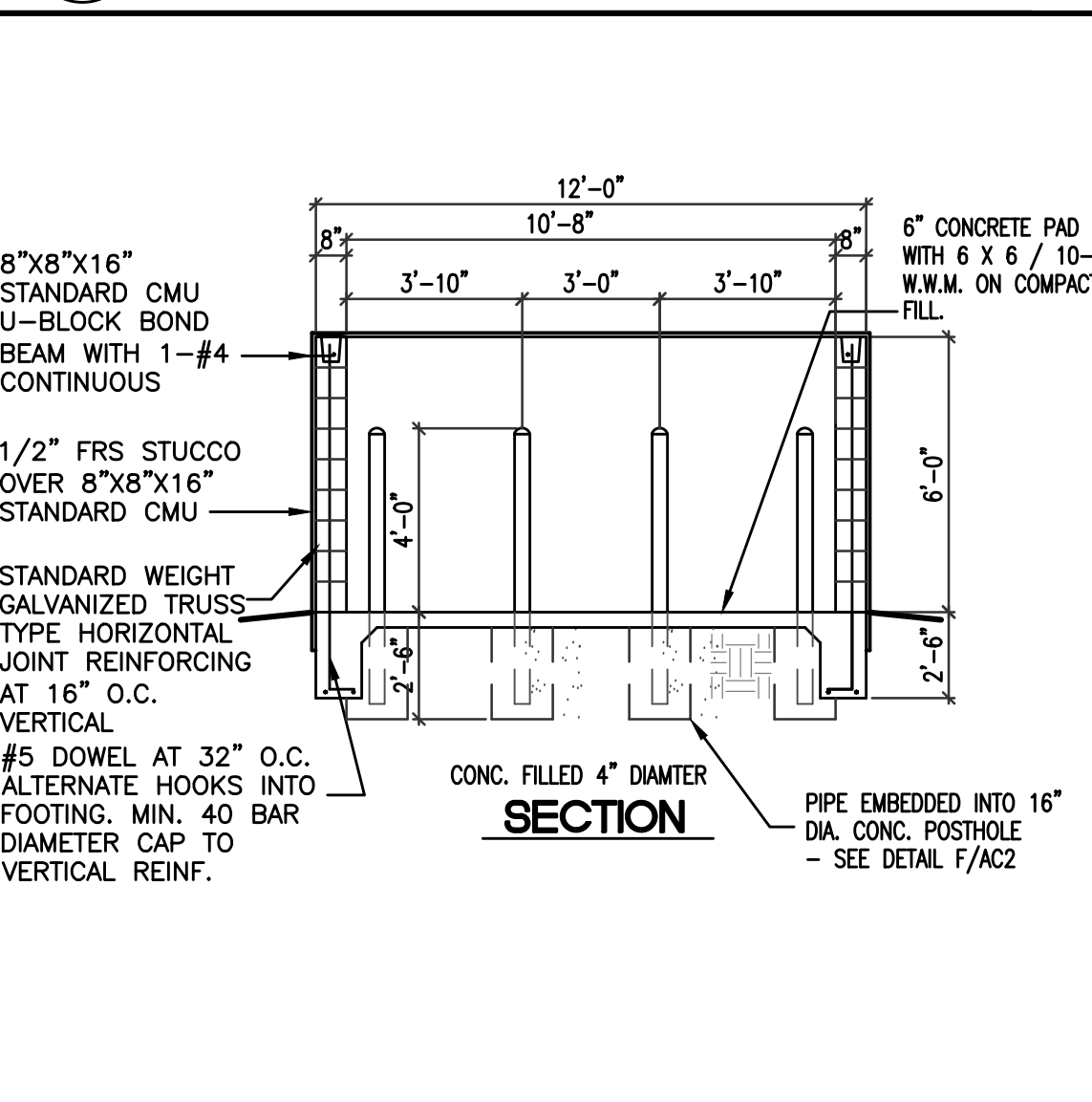
B TRASH ENCLOSURE SECTION AC2 NOT TO SCALE
