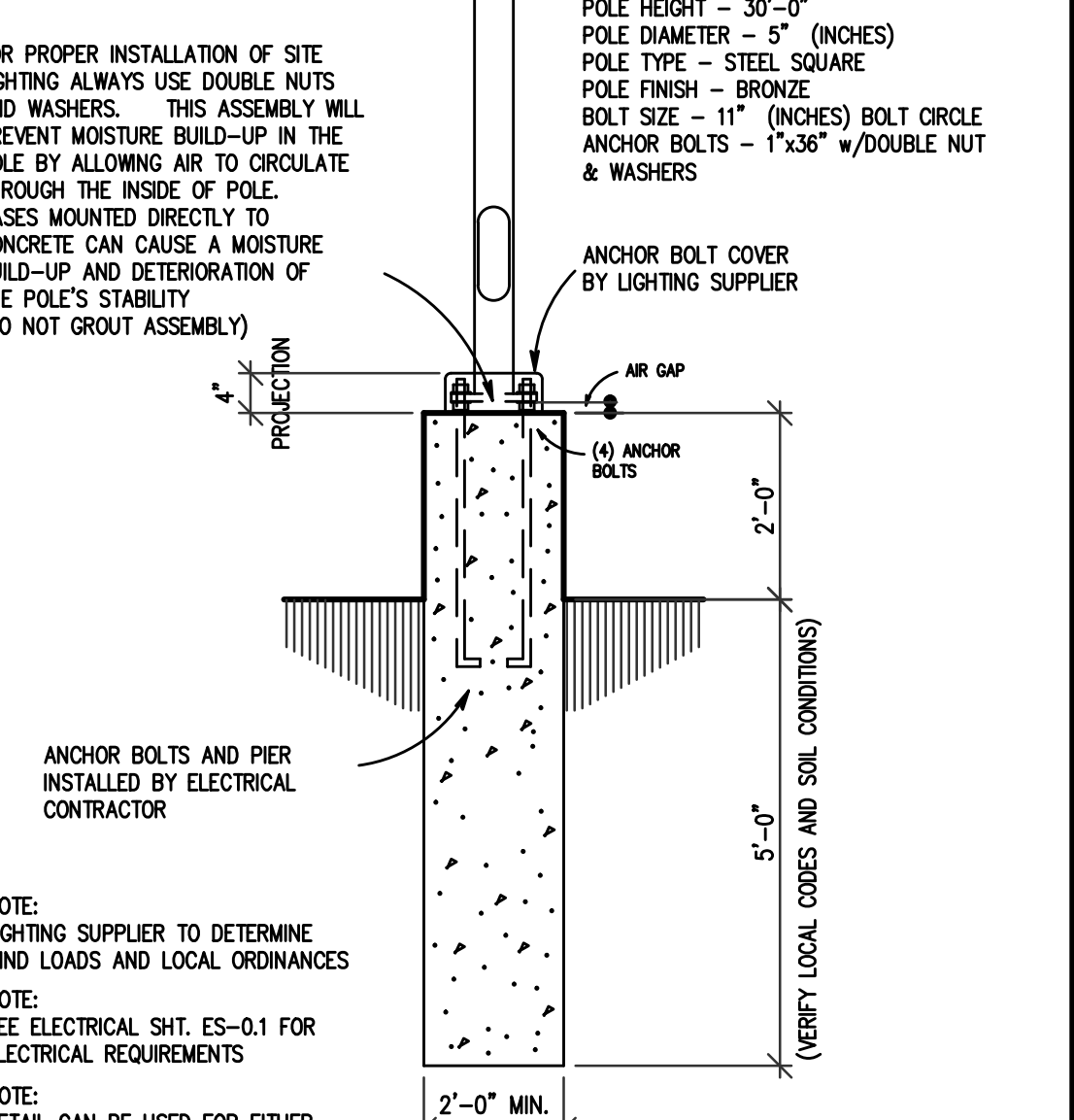
E EXTERIOR POLE LIGHTS AC2 NOT TO SCALE
