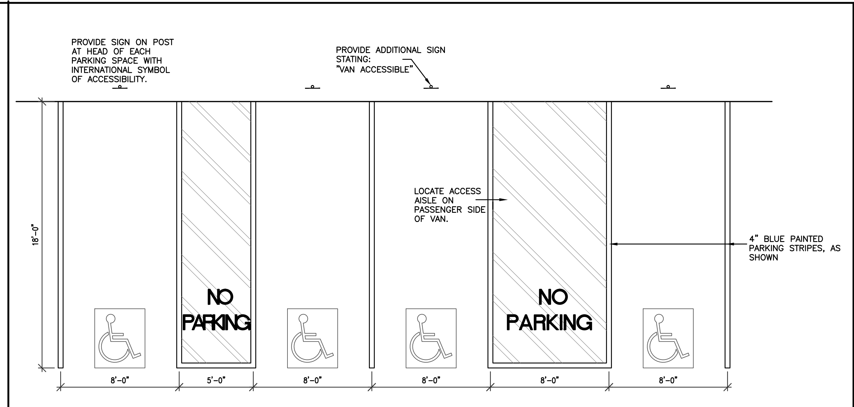
M HC PARKING SPACE REQUIREMENTS AC2 NOT TO SCALE
