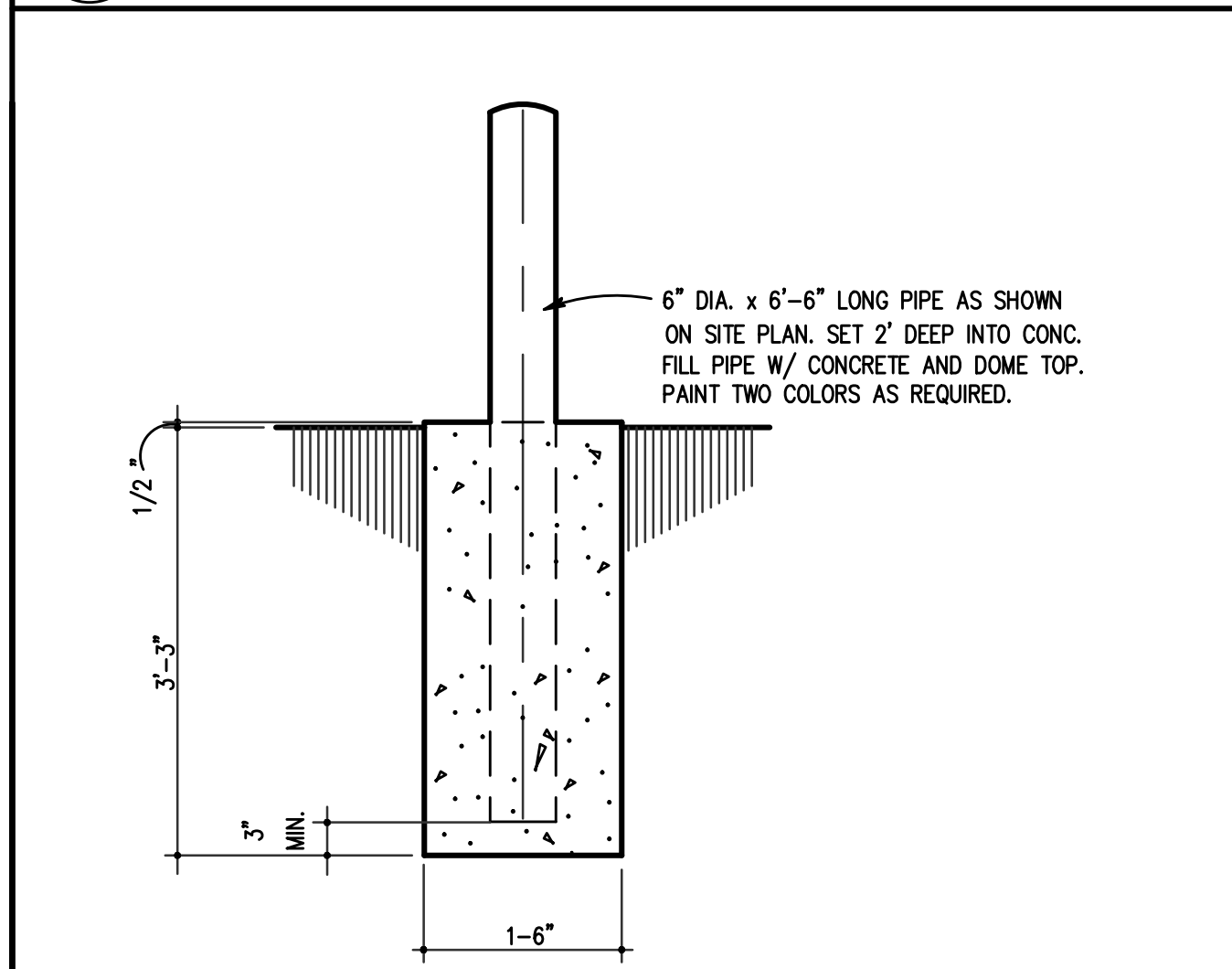
F TYP. BOLLARD AC2 NOT TO SCALE
