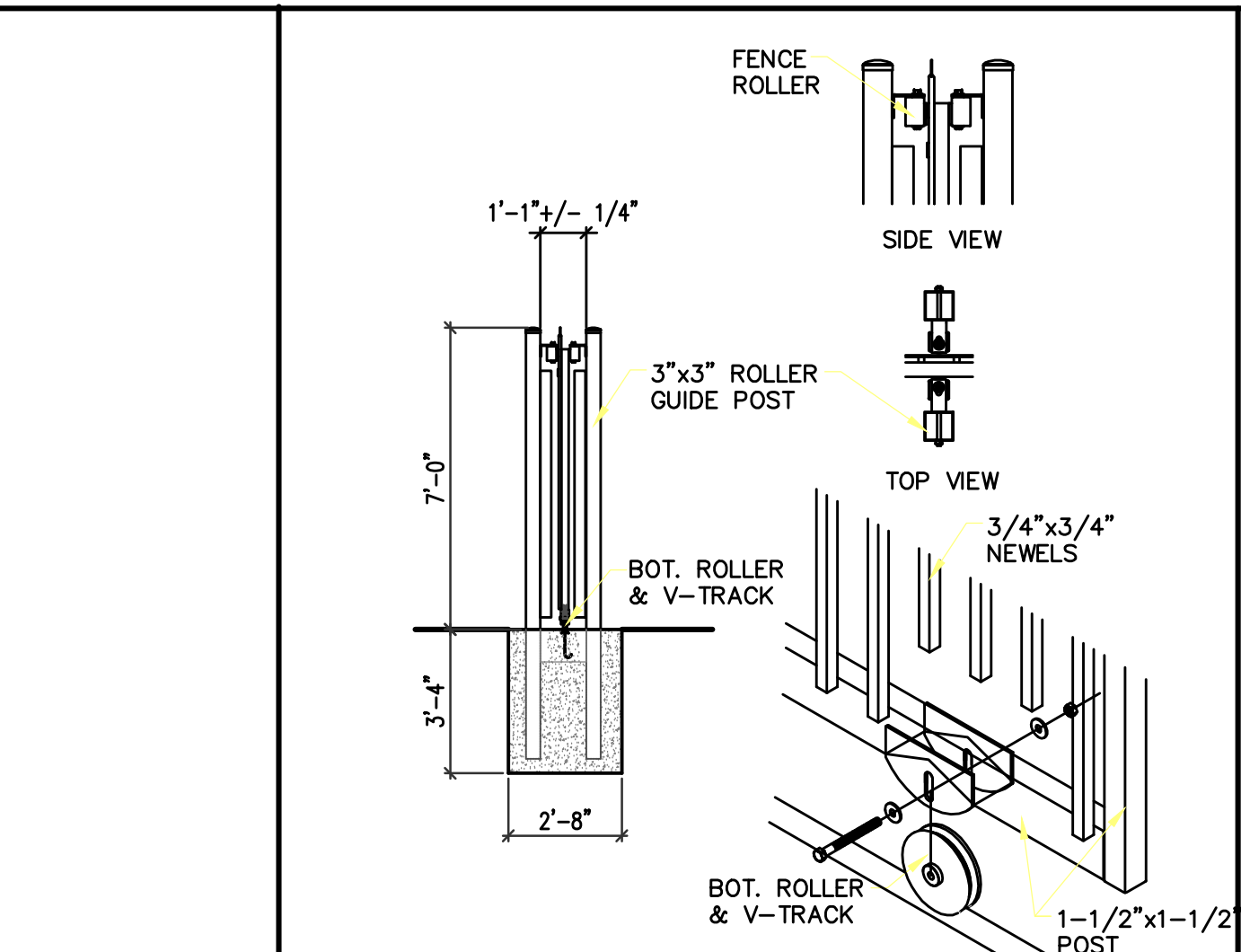
J SLIDING GATE DETAIL AC2 NOT TO SCALE
