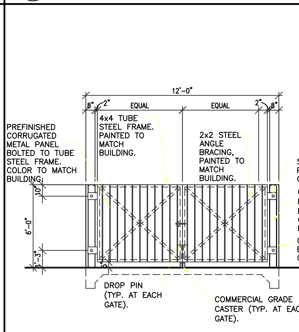
C TRASH ENCLOSURE AC2 NOT TO SCALE
