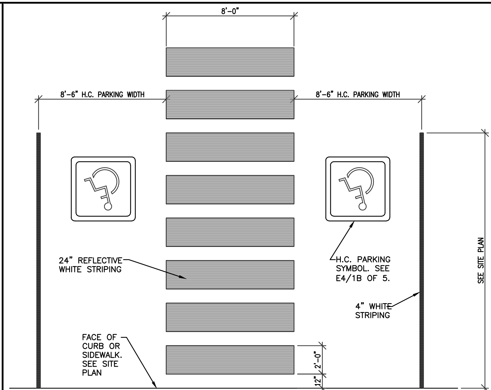
L HC PARKING ACCESS STRIPING PLAN AC2 NOT TO SCALE
