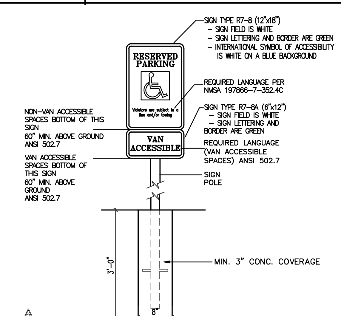
G TYP. H.C. SIGNAGE AC2 NOT TO SCALE
