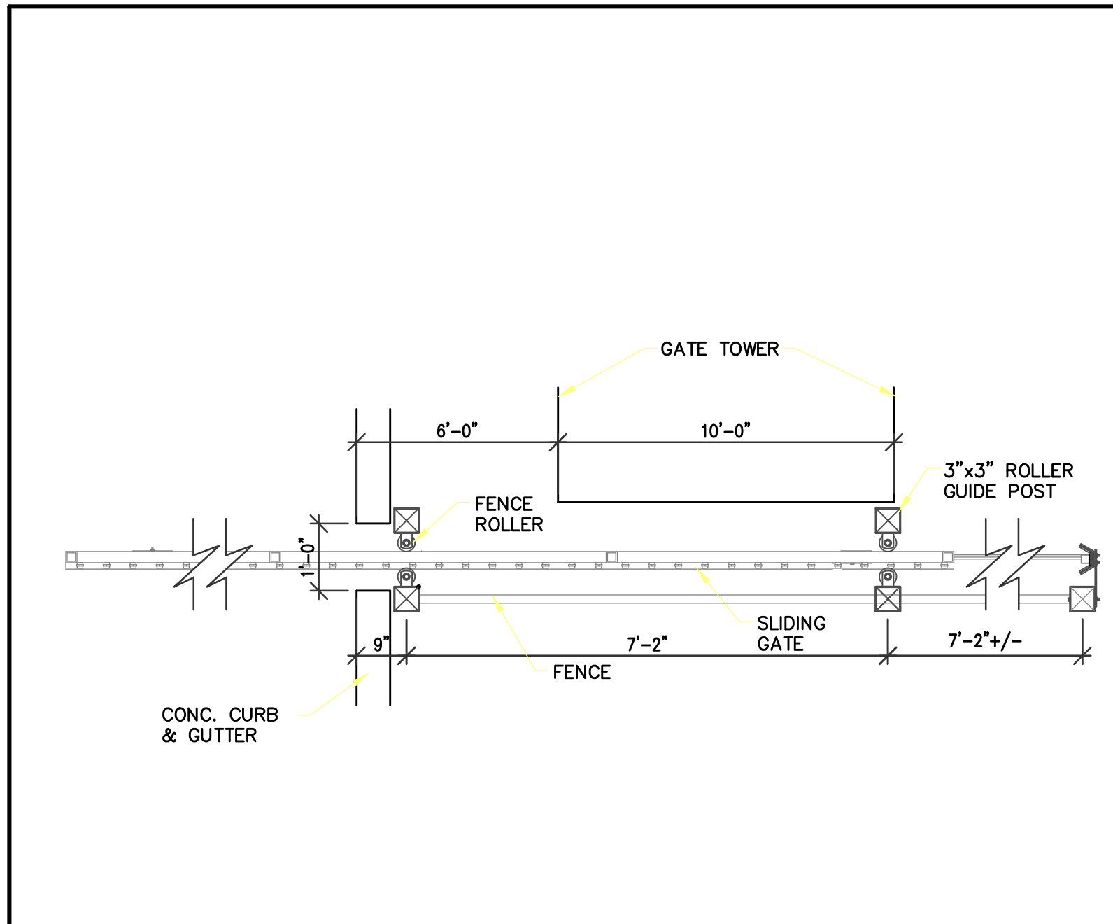
K SLIDING GATE DETAIL AC2 NOT TO SCALE
