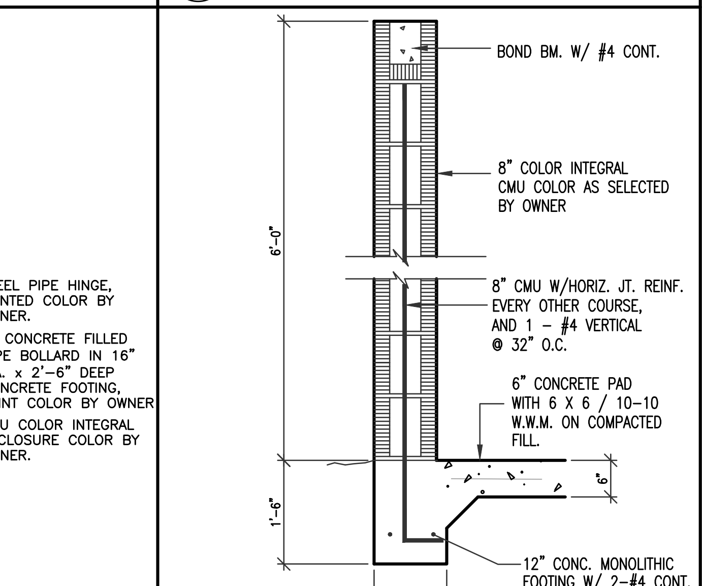
D CMU WALL DETAIL AT DUMPSTER AC2 NOT TO SCALE
