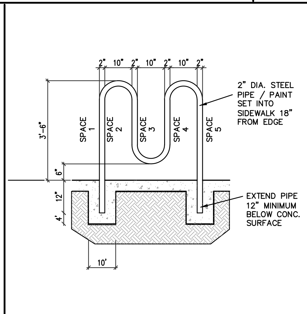
H BICYCLE RACK AC2 NOT TO SCALE
