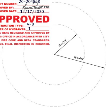
FIRE APPARATUS TURNING RADIUS 1"=20'
