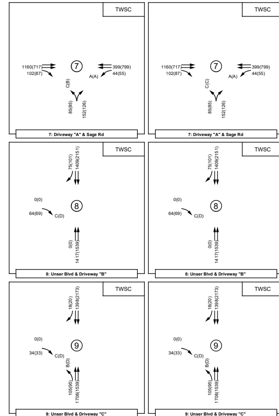
Unser and Sage Development 2035 (Driveways A-C) LOS / Volume Analysis Map
