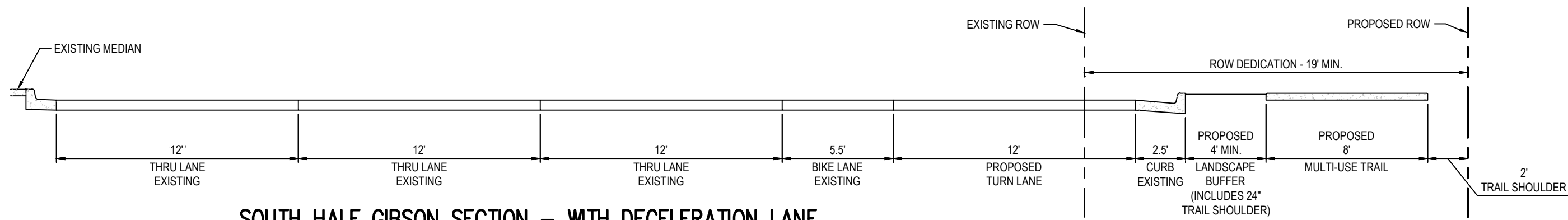
SOUTH HALF GIBSON SECTION - WITH DECELERATION LANE NOT TO SCALE
