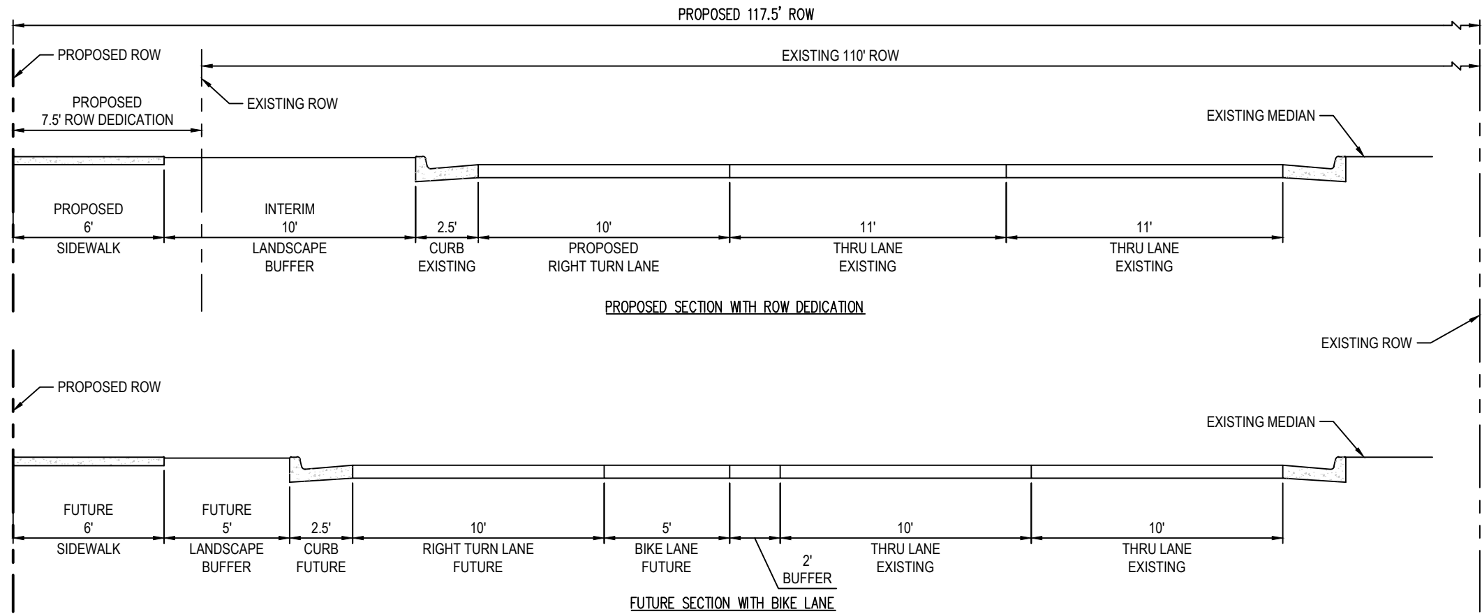
PROPOSED YALE BOULEVARD ROW SECTION NOT TO SCALE
