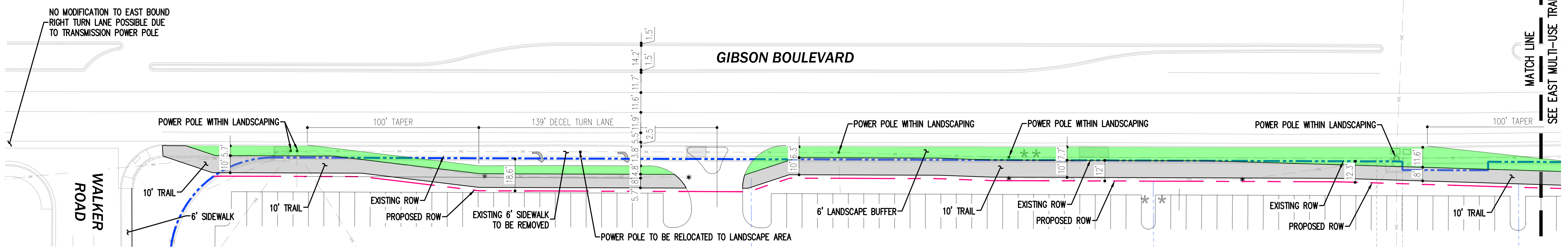
WEST MULTI-USE TRAIL SCALE: 1"=30'
