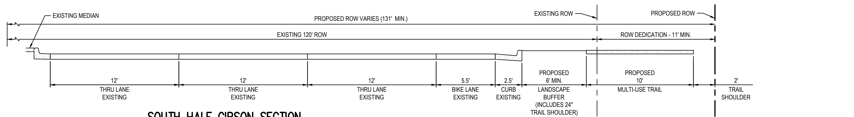
SOUTH HALF GIBSON SECTION NOT TO SCALE
