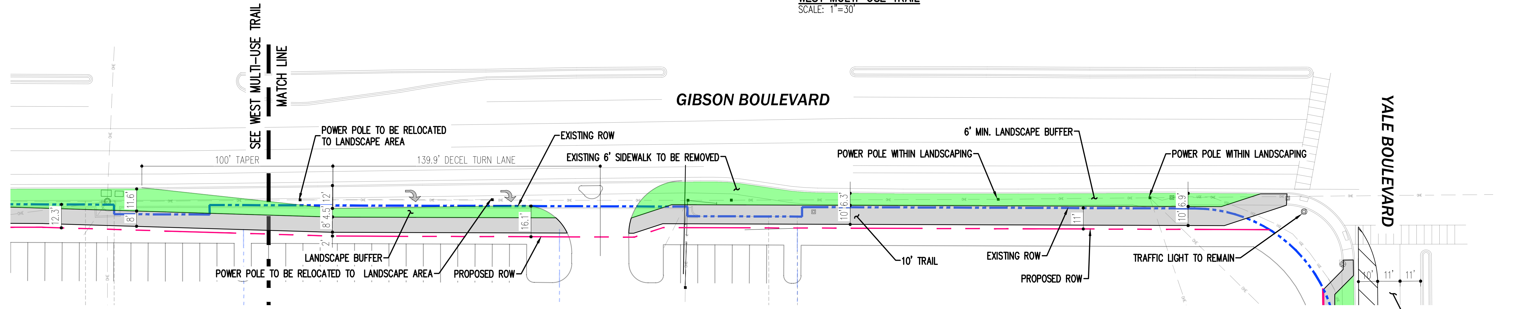
EAST MULTI-USE TRAIL SCALE: 1"=30'
