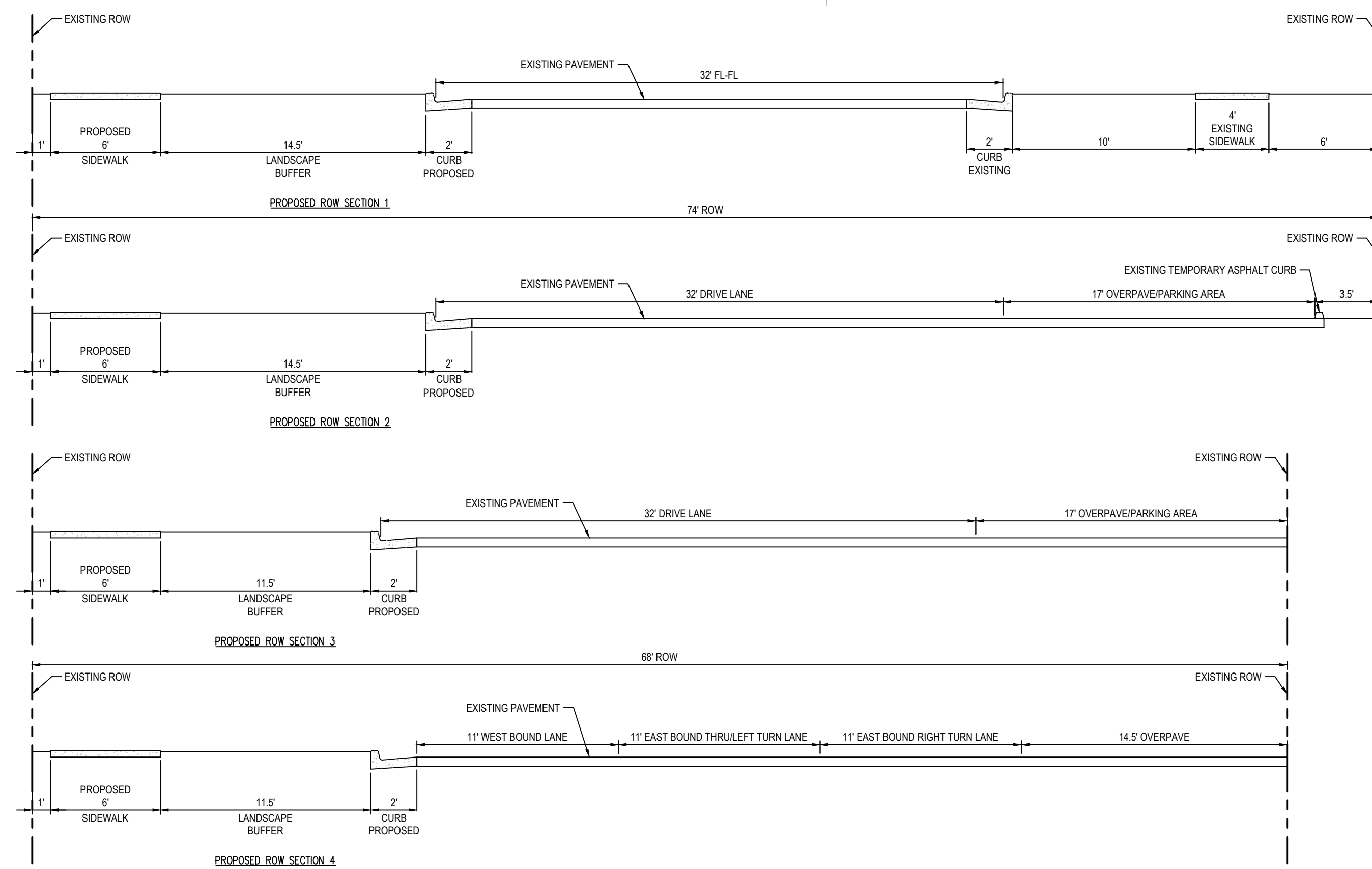
PROPOSED MILES ROAD ROW SECTION NOT TO SCALE
