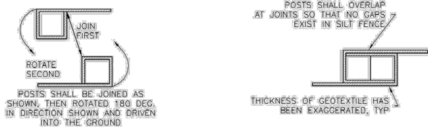
SECTION A
