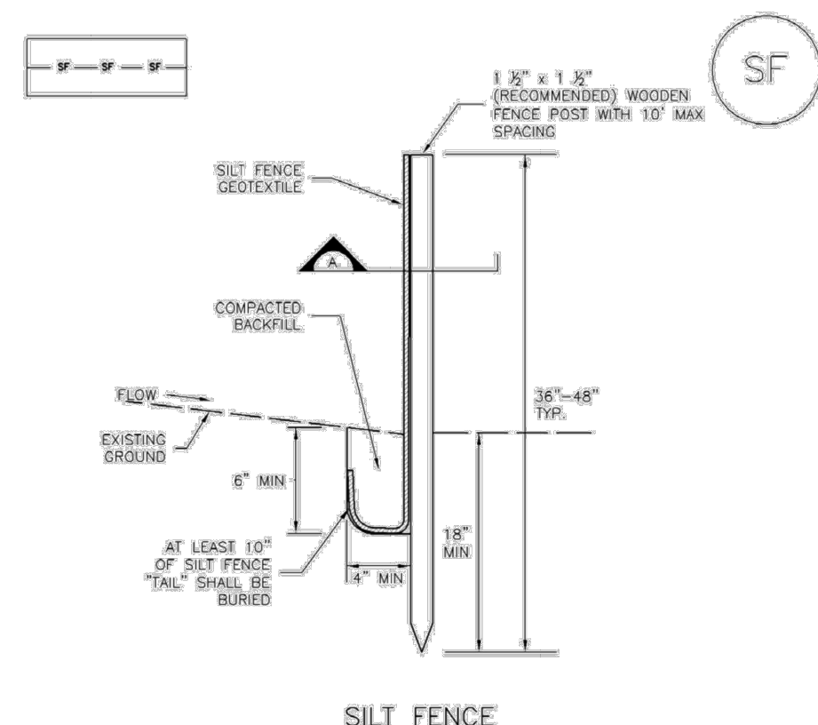
SILT FENCE
