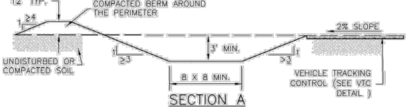
SECTION A
