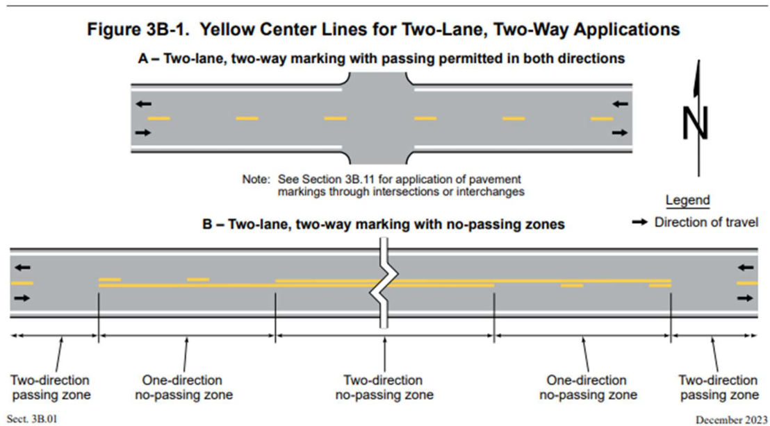
Figure 16: MUTCD Section 3B-01 Yellow Center Line Pavement Markings
