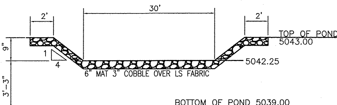
POND B-1 EMERGENCY SPILLWAY DETAIL NTS
