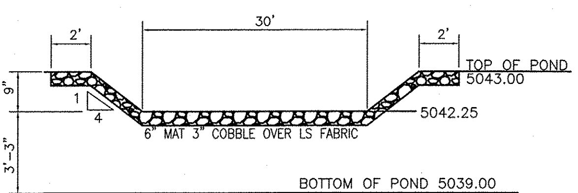
POND B-2 EMERGENCY SPILLWAY DETAIL NTS
