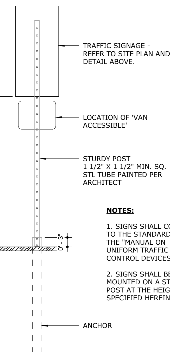
A5 TRAFFIC SIGNAGE 3/4" = 1'-0"
