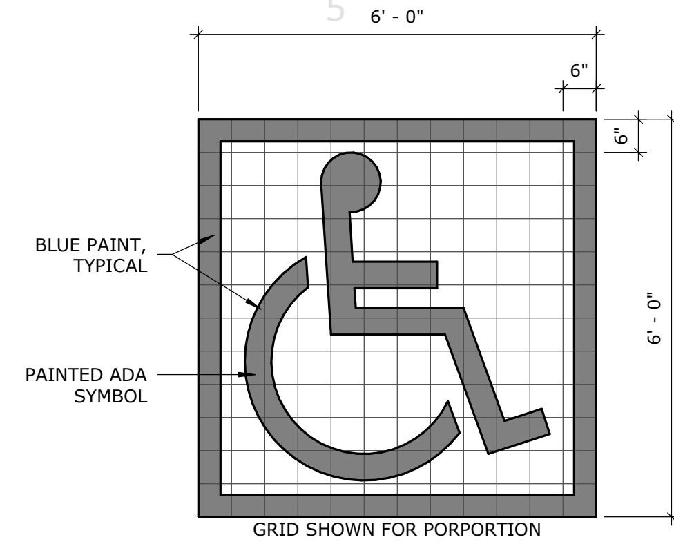
E5 PAINTED HC SYMBOL 1/2" = 1'-0"
