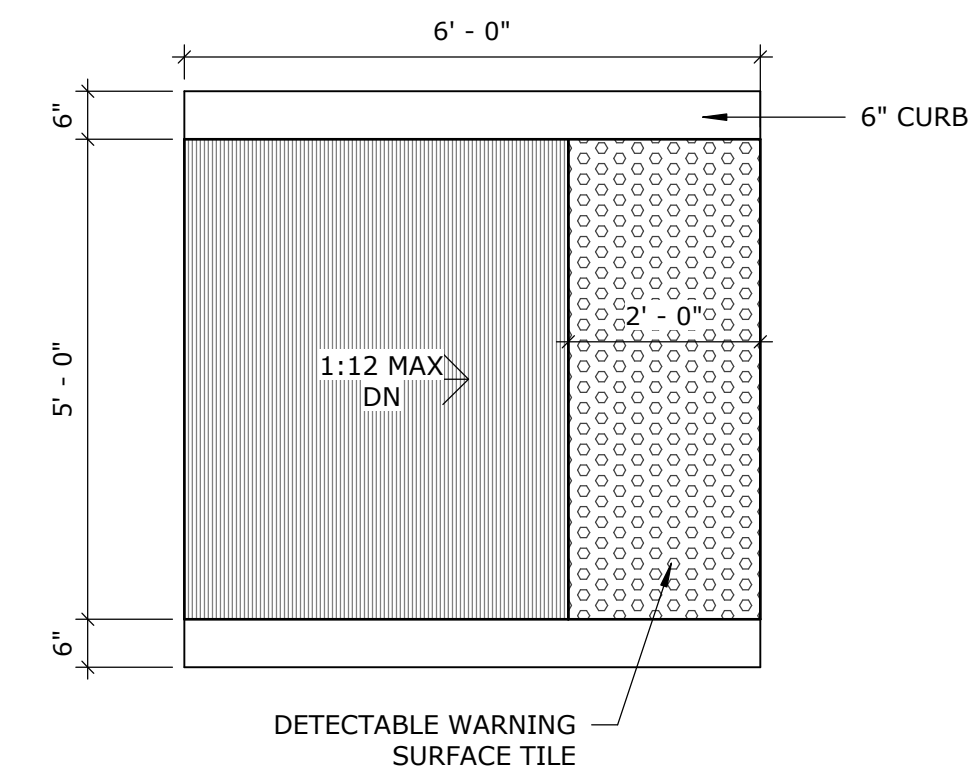
D5 HC ACCESS RAMP 1/2" = 1'-0"
