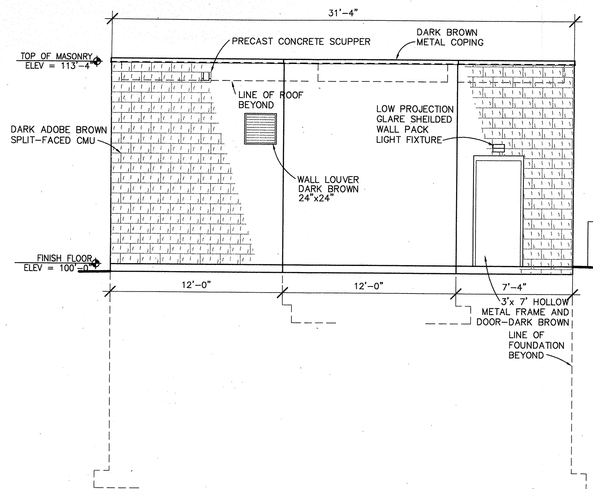
NORTH ELEVATION 1/4"=1'-0"
