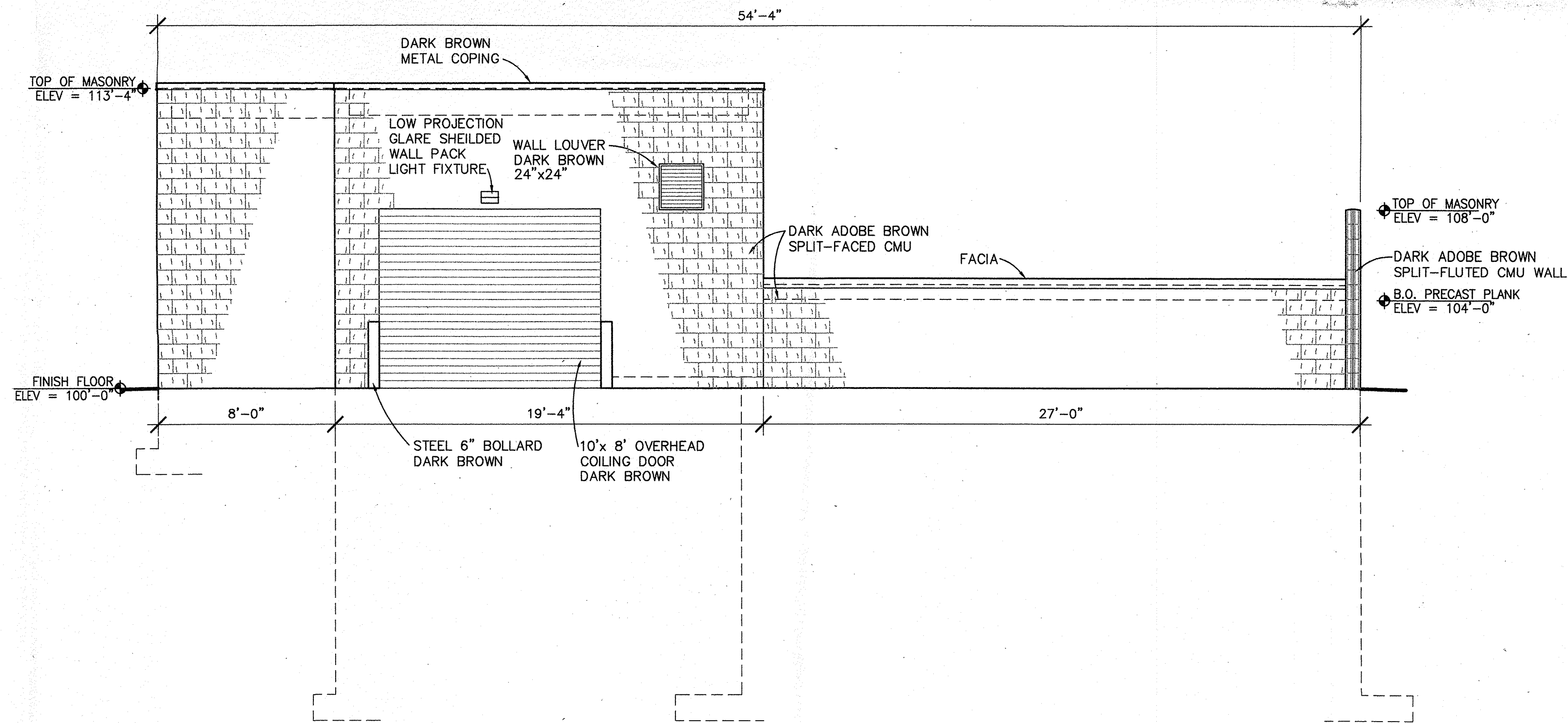
WEST ELEVATION 1/4"=1'-0"
