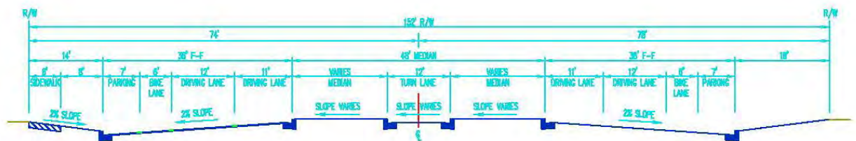
UNIVERSITY BLVD. – 152' ROW NOT TO SCALE
