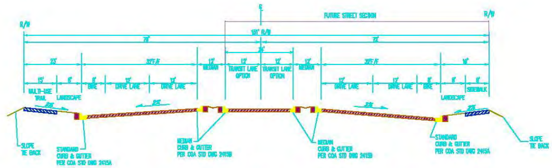
© TYPICAL STREET SECTION – MESA DEL SOL BLVD N.T.S.
